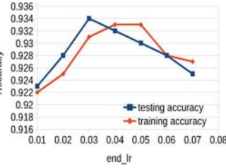
Figure 9: learning rate
