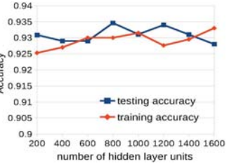
Figure 10: hidden units
