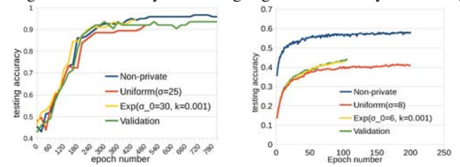
Figure 14: Accuracy (Cancer)
