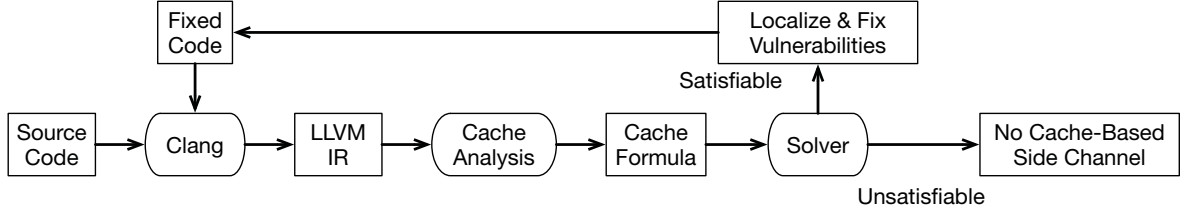
Figure 2: System flow of CaSym.
