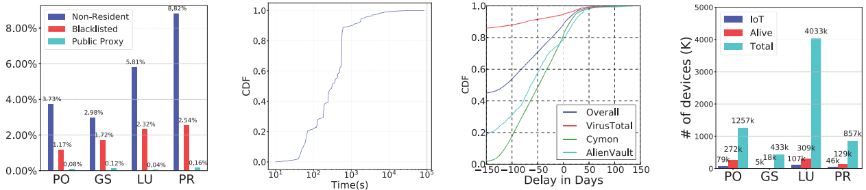
(a) % of non-residential, blacklisted, published proxy IPs in RESIP services
