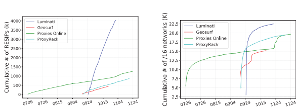
(a) Cumulative number of RESIPs. (b) Cumulative number of /16 RESIPs.
