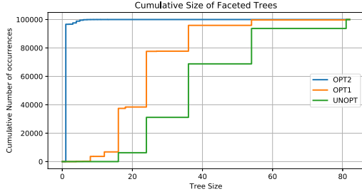
Fig. 13. Data-optimisations on faceted values (computing overlapping times)
