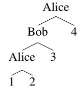
Fig. 5. A difficult to shrink tree
