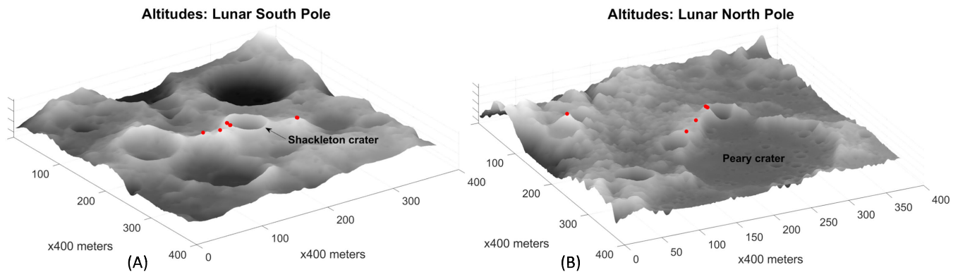
FIGURE 2. Stereographic projection of lunar poles topography from latitude \mp 87.5 to \mp 90 . (A) Lunar south pole. (B) Lunar north pole. Database recovered from [18]. Red dots indicate some of the highly illuminated areas provided in Table 2 [15]–[17].
