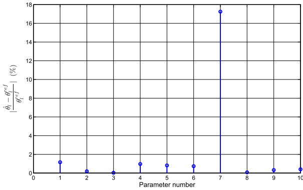
FIGURE 12. OP4: final values of |\hat{\theta}_1 - \theta_1^{ref}| / \theta_1^{ref} (in %) with \theta^{ref} = \hat{\theta}_1 . The first 10 components are considered; the others are treated separately [16].
