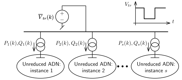
FIGURE 4. Disturbance simulation on randomized instances of the ADN model.
