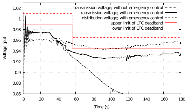
FIGURE 25. IEEE Nordic test system with ADN equivalents. Voltages at bus 1041 and on the distribution side of a transformer connected to bus 1041.
