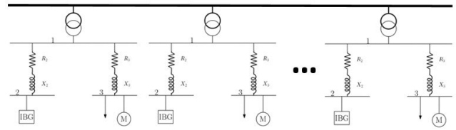
FIGURE 21. Connection of multiple ADN equivalents to a transmission bus (in the central region of the IEEE Nordic test system).
