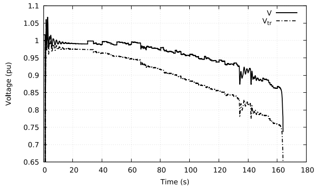
FIGURE 16. IEEE Nordic test system: transmission and distribution voltages.
