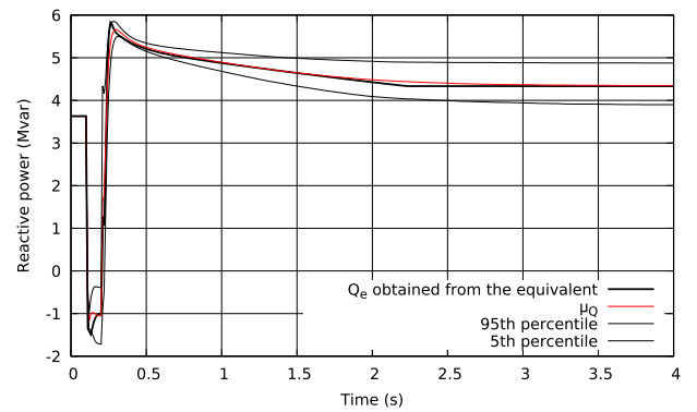
FIGURE 9. Reactive power flowing into the equivalent, compared to the average and the percentiles of the randomized responses shown in Fig. 7.
