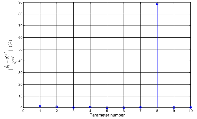
FIGURE 10. OP3: final values of |\hat{\theta}_i - \theta_i^{ref}| / \theta_i^{ref} (in %), with \theta^{ref} = \hat{\theta}_1 . The first 10 components are considered; the others are treated separately [16].
