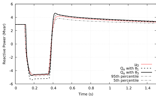
FIGURE 13. OP4: reactive power response of the equivalent to a severe voltage dip, using \hat{\theta}_1 and \hat{\theta}_3 , respectively.
