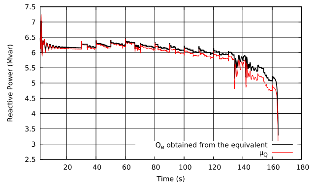
FIGURE 18. Reactive power flow into the ADN and its equivalent. Disconnection of IBGs not modelled.
