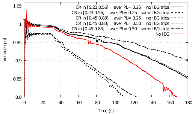
FIGURE 24. IEEE Nordic test system with ADN equivalents. Voltage at bus 1041.
