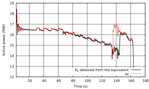
FIGURE 19. Active power flow into the ADN and its equivalent. Disconnection of IBGs taken into account.
