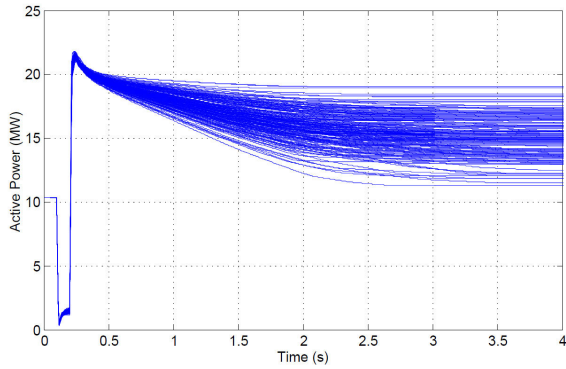
FIGURE 6. Randomized evolutions of the active power flowing into the ADN, in response to a voltage dip of 0.8 pu lasting 100 ms (applied at t = 0.1 s).
