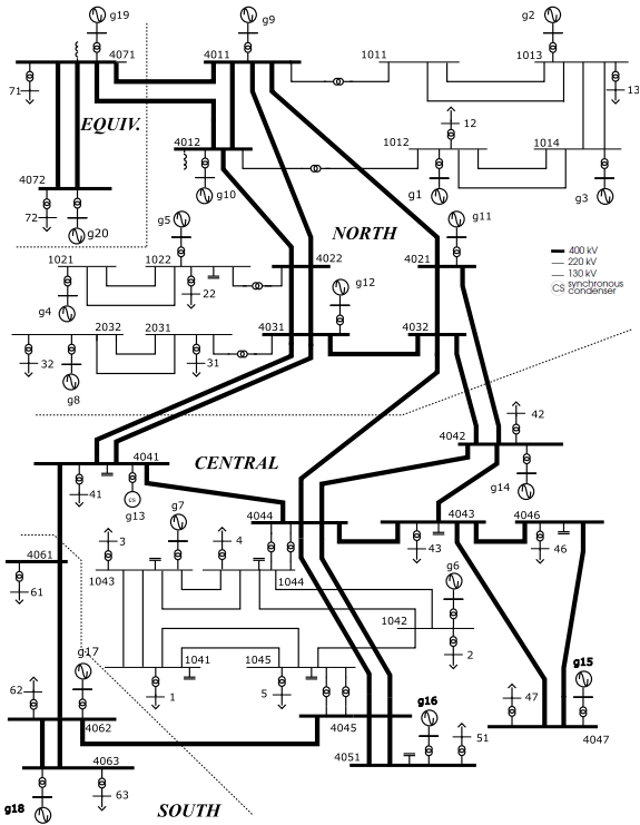
FIGURE 15. IEEE Nordic test system [30].
