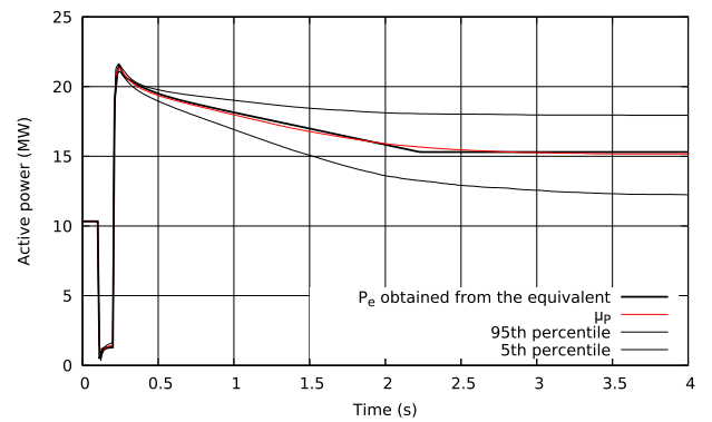
FIGURE 8. Active power flowing into the equivalent, compared to the average and the percentiles of the randomized responses shown in Fig. 6.
