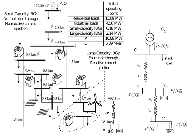
FIGURE 14. Variant of the CIGRE MV distribution network benchmark (left) and its dynamic equivalent (right).
