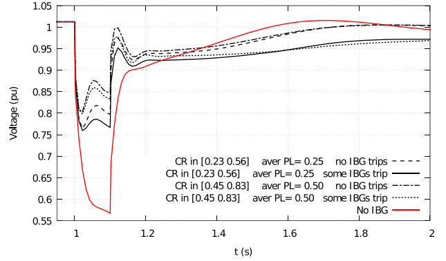
FIGURE 23. IEEE Nordic test system with ADN equivalents. Voltage at bus 1041. Disconnection of IBGs taken into account.
