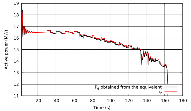
FIGURE 17. Active power flow into the ADN and its equivalent. Disconnection of IBGs not modelled.
