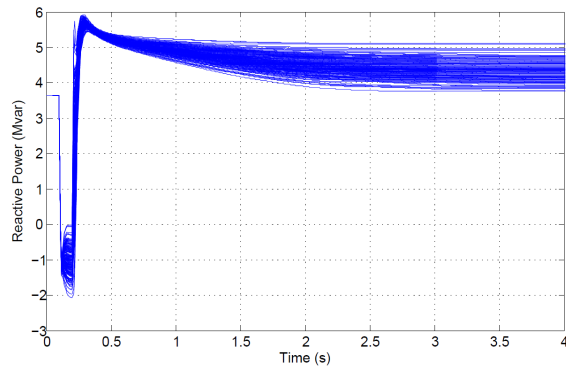
FIGURE 7. Randomized evolutions of reactive power flowing into the ADN, in response to a voltage dip of 0.8 pu lasting 100 ms (applied at t = 0.1 s).
