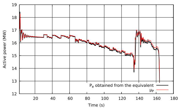
FIGURE 20. Active power flow into the ADN and its equivalent. Disconnection of IBGs taken into account and LVRT curve of the equivalent IBG adjusted.
