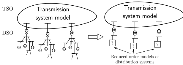
FIGURE 1. Replacing ADNs by their equivalents.
