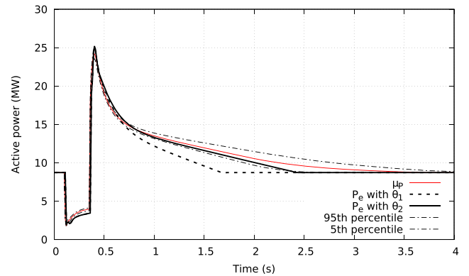
FIGURE 11. OP3: active power response of the equivalent to a severe voltage dip, using \hat{\theta}_1 and \hat{\theta}_2 , respectively.
