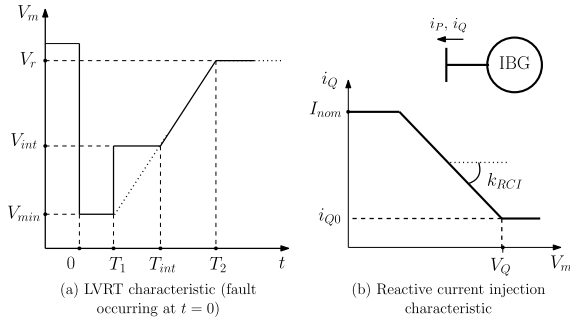
FIGURE 3. IBG controls responding to large voltage deviations.
