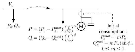
FIGURE 2. Load model: decomposition into exponential and motor parts [16].
