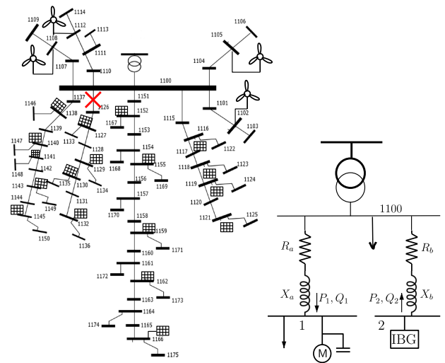
FIGURE 5. Unreduced ADN (left) and its grey-box dynamic equivalent (right).
