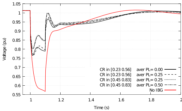
FIGURE 22. IEEE Nordic test system with ADN equivalents. Voltage at bus 1041. Disconnection of IBGs not taken into account.
