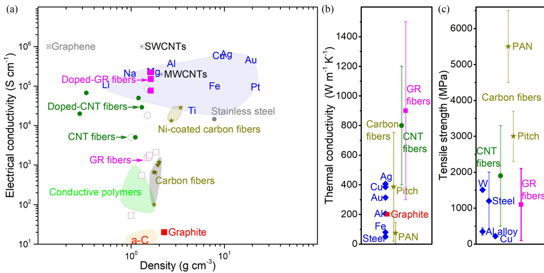
FIGURE 4. (a) Electrical, (b) thermal conductivities, and (c) tensile strength of CNT- (dark green) and graphene-fibers (magenta) compared to carbon fibers (brown) and some metals (blue). Original work from [36], reproduced under CC-BY-4.0.
