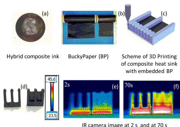
FIGURE 5. (a–c) Schematic of buckypaper heat sink. (a) Composite ink obtained by epoxy filled with graphite-nanoplatelets and carbon fiber. (b) Free standing carbon nanotube films, or buckypaper (BP). (c) Printed heat sink using composite ink, with BP incorporated. (d) Heat sinks without (on the left) and with BP (on the right). (e–f) Heat dissipation as measured from IR camera of two heat sinks at different time frames. Reprinted with permission from [58]. Copyright 2021 American Chemical Society. Original work has been modified with permission.
