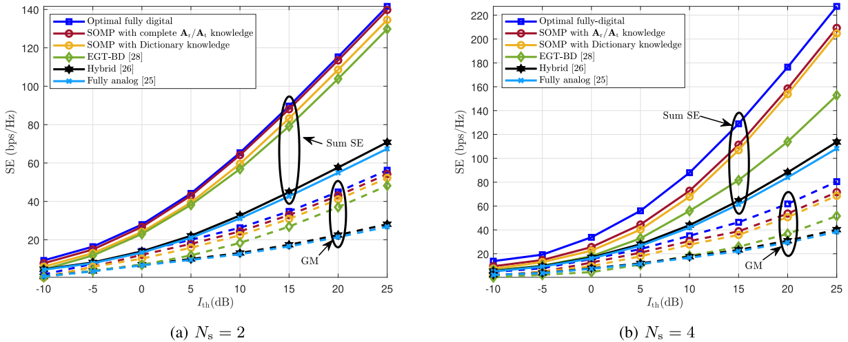
FIGURE 3. SE versus I_{th} of different TPC/RC solutions for a 8 \times 128 mmWave MU MIMO CR system with M = 8 , M_r = 2N_s , M_t = MM_r .
