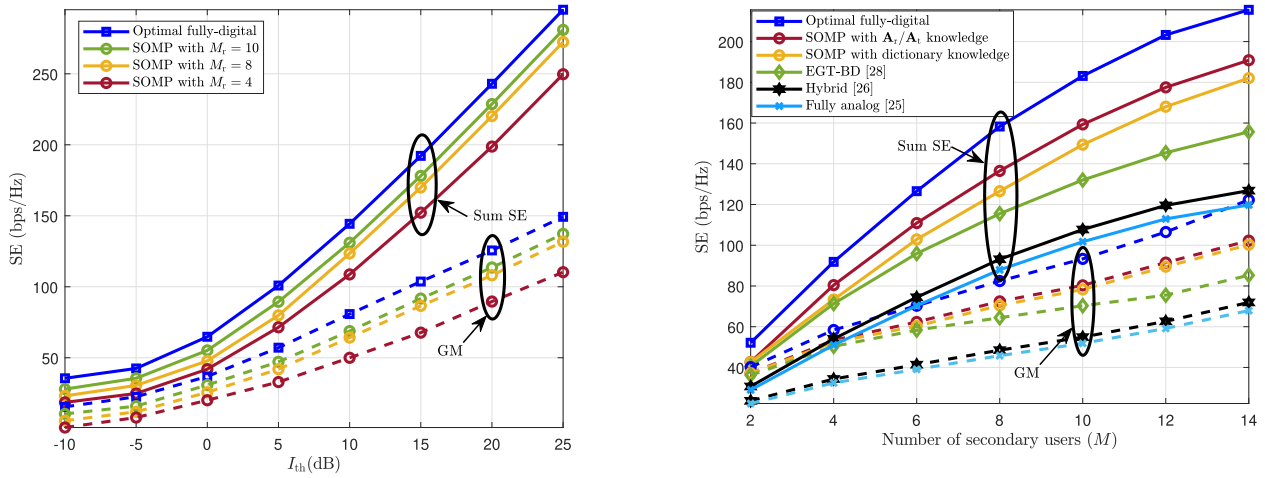
FIGURE 7. SE attained by different TPC/RC solutions in a 16 \times 256 mmWave MU MIMO CR system where M increases from 2 to 14, I_{th} = 5 dB and N_s = 4 .
