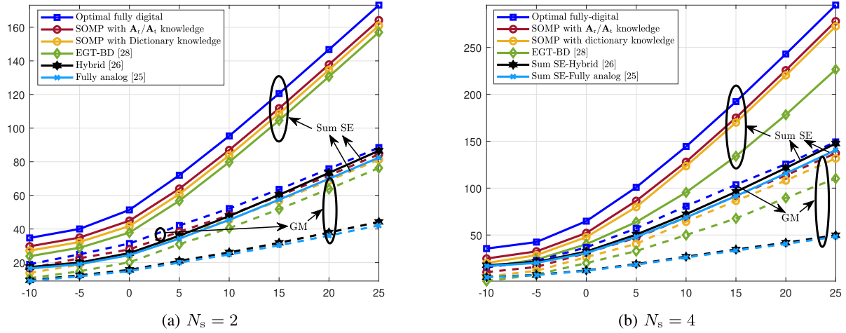
FIGURE 4. SE versus I_{th} of different TPC/RC solutions for a 16 \times 256 mmWave MU MIMO CR system with M = 8 , M_r = 2N_s , M_t = MM_r .
