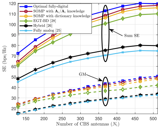
FIGURE 8. SE attained by different TPC/RC solutions where the number of CBS antennas ( N_t ) varies from 128 to 512, N_r = 8 , M = 8 , I_{th} = 5 dB and N_s = 2 .
