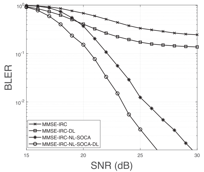
FIGURE 10. BLER performance as a function of SNR for various schemes, for the case of N_r = 4 RAs, N_u = 4 user TAs, N_i = 1 interfering user TA, K' = 2048 information bits, L_{max} = 4 slicing value, coding rate R = 1/2 , SIR = 10 dB, BG = 2, N_c = 64 subcarriers when using 16-QAM modulation for communication over a frequency selective fading channel with L = 4 channel taps. For the NL-SOCA tree search in the case of MMSE-IRC-NL-SOCA and MMSE-IRC-NL-SOCA-DL schemes, the number of child nodes created in each layer is M = [4 \ 1 \ 1 \ 1] and the number of surviving child nodes in each layer is K = [4 \ 4 \ 4 \ 4] . The number of outer iterations performed between the NL-SOCA detector and LDPC decoder is I_{outer} = 4 .
