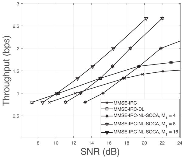
FIGURE 13. Throughput as a function of the SNR where a BLER of 10^{-1} is achieved, for the case of N_r = 4 RAs, N_u = 4 user TAs, N_i = 1 interfering user TA, K' = 2048 information bits, L_{\max} = 4 slicing value, SIR = 0 dB, BG = 2, N_c = 64 subcarriers, when using 16-QAM modulation for communication over a frequency selective fading channel with L = 4 channel taps. For the NL-SOCA tree search in the case of the MMSE-IRC-NL-SOCA scheme, the number of child nodes created in each layer is M = [M_1 \ 1 \ 1 \ 1] and the number of surviving child nodes in each layer is K = [M_1 \ M_1 \ M_1 \ M_1] , where M_1 = 4, 8 and 16 are considered. The number of outer iterations performed between the NL-SOCA detector and LDPC decoder is I_{\text{outer}} = 4 .
