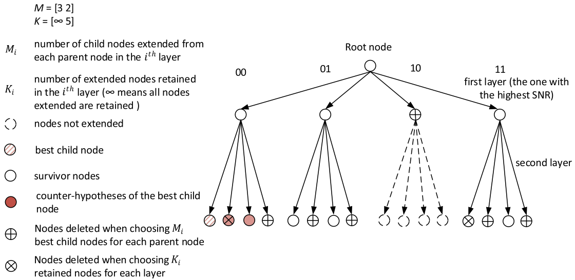
FIGURE 4. Example of tree search in the NL-SOCA detector for the case m = 2 bits mapped into the QPSK modulated symbol transmitted in each of N_u = 2 layers using N_u = 2 transmit antennas.
