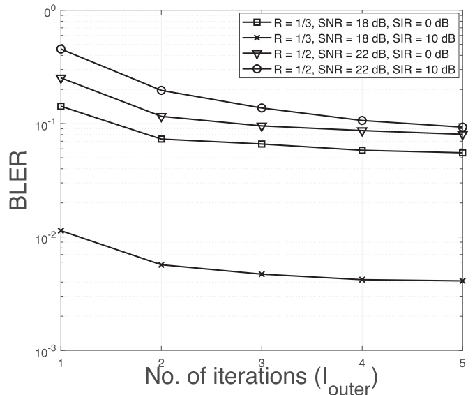
FIGURE 8. BLER performance as a function of the number of iterations performed between the NL-SOCA detector and LDPC decoder in the MMSE-IRC-NL-SOCA scheme, for the case of N_r = 4 RAs, N_u = 4 user TAs, N_i = 1 interfering user TA, K' = 2048 information bits, L_{\text{max}} = 4 clipping value, BG = 2 , N_c = 64 subcarriers when using 16-QAM modulation for communication over a frequency selective fading channel with L = 4 channel taps. In the NL-SOCA tree search, the number of child nodes created at each layer is M = [M_1 \ 1 \ 1 \ 1] and the number of surviving child nodes in each layer is K = [M_1 \ M_1 \ M_1 \ M_1] . Plots are provided for various combinations of coding rates R , SNR, and SIR.
