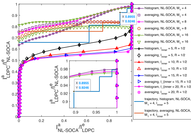
FIGURE 6. NL-SOCA and LDPC EXIT functions of the LDPC-coded MMSE-IRC-NL-SOCA scheme, for the case of N_r = 4 receive antennas, N_u = 4 desired user transmit antennas, N_i = 1 interfering user transmit antenna, K' = 2048 information bits, an LDPC coding rate of R = 1/2 using base graph 2, an SNR of 22 dB, an SIR of 0 dB, N_c = 64 subcarriers, when using 16-QAM modulation for communication over a frequency selective fading channel with L = 4 channel taps. For the NL-SOCA tree search, the number of child nodes extended in each layer is M = [M_1 \ 1 \ 1] and the number of survivor child nodes retained in each layer is K = [M_1 \ M_1 \ M_1 \ M_1] , where M_1 \in \{4, 8, 16\} .
