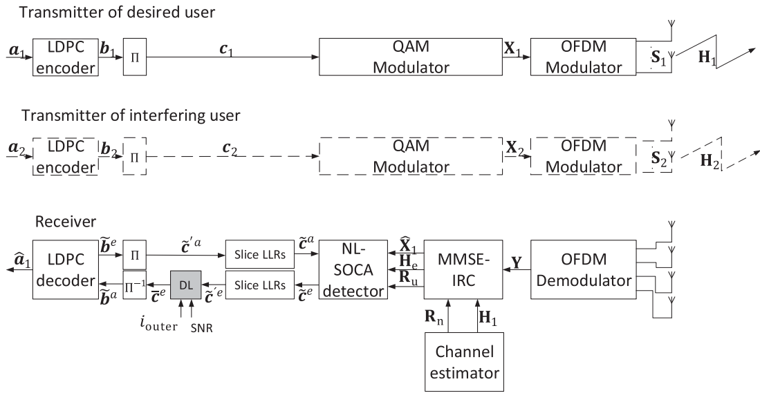
FIGURE 3. Schematic of the transmitter and receiver for the proposed LDPC-coded MMSE-IRC-NL-SOCA/MMSE-IRC-NL-SOCA-DL scheme. The dashed lines correspond to interfering users and the grey-shaded block is specific to the MMSE-IRC-NL-SOCA-DL scheme.
