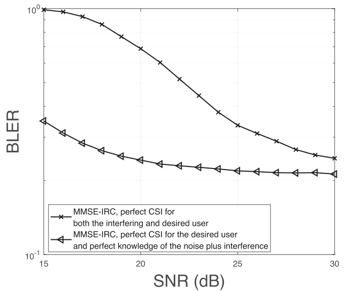
FIGURE 2. Comparison between the assumption of perfect channel state information for both the interfering and desired users, with the assumption of perfect knowledge of the interference plus noise signal for the case of N_r = 4 RAs, N_u = 4 user TAs, N_i = 1 interfering user TA, K' = 2048 information bits, L_{\max} = 4 slicing value, coding rate R = 1/2 , SIR = 10 dB, BG = 2, N_c = 64 subcarriers, when using 16-QAM modulation for communication over a frequency selective fading channel with L = 4 channel taps.
