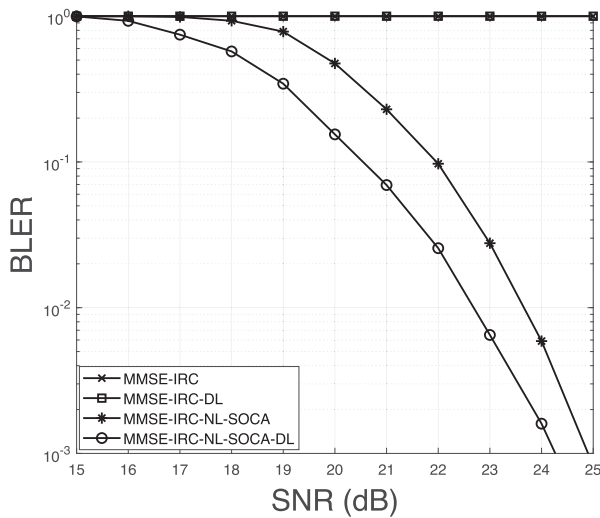
FIGURE 9. BLER performance as a function of SNR for various schemes, for the case of N_r = 4 RAs, N_u = 4 user TAs, N_i = 1 interfering user TA, K' = 2048 information bits, L_{max} = 4 slicing value, coding rate R = 1/2 , SIR = 0 dB, BG = 2, N_c = 64 subcarriers, when using 16-QAM modulation for communication over a frequency selective fading channel with L = 4 channel taps. For the NL-SOCA tree search in the case of the MMSE-IRC-NL-SOCA and MMSE-IRC-NL-SOCA-DL schemes, the number of child nodes created at each layer is M = [4 \ 1 \ 1 \ 1] and the number of surviving child nodes in each layer is K = [4 \ 4 \ 4 \ 4] . The number of outer iterations performed between the NL-SOCA detector and LDPC decoder is I_{outer} = 4 .
