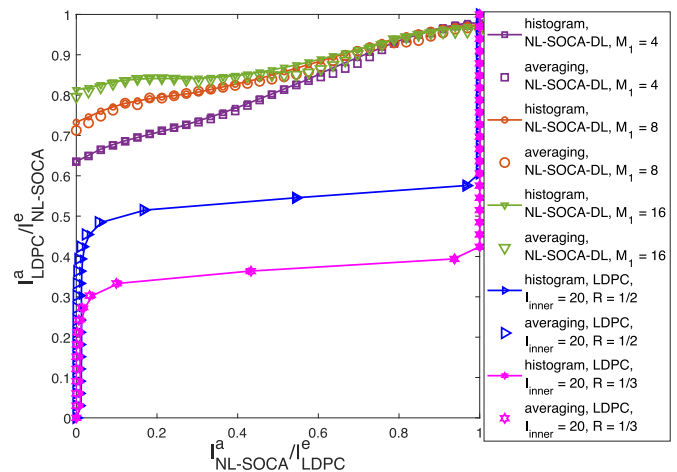
FIGURE 7. NL-SOCA-DL and LDPC EXIT functions for the LDPC-coded MMSE-IRC-NL-SOCA-DL scheme for the case of N_r = 4 RAs, N_u = 4 desired user TAs, N_i = 1 interfering user TA, K' = 2048 information bits, base graph 2, an SNR of 22 dB, an SIR of 0 dB, N_c = 64 subcarriers when using 16-QAM modulation for communication over a frequency selective fading channel with L = 4 channel taps. In the NL-SOCA tree search, the number of extended child nodes in each layer M = [M_1 \ 1 \ 1] and the number of survived child nodes in each layer K = [M_1 \ M_1 \ M_1 \ M_1] .
