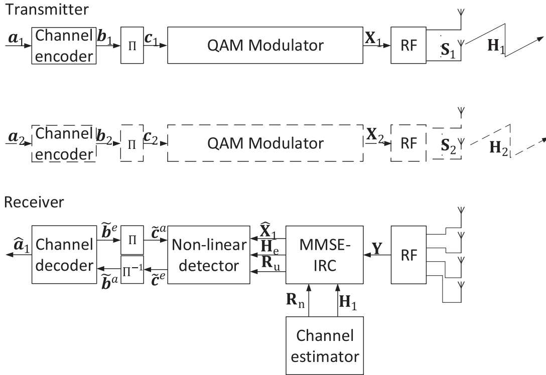
FIGURE 1. Schematic of a system contaminated by an interfering user, where the receiver combines the MMSE-IRC with a NL detector.
