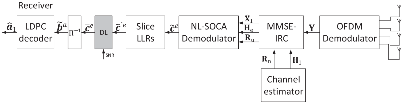
FIGURE 5. Schematic of the receiver for the MMSE-IRC/MMSE-IRC-DL scheme. The grey shaded block is specific to the MMSE-IRC-DL scheme.
