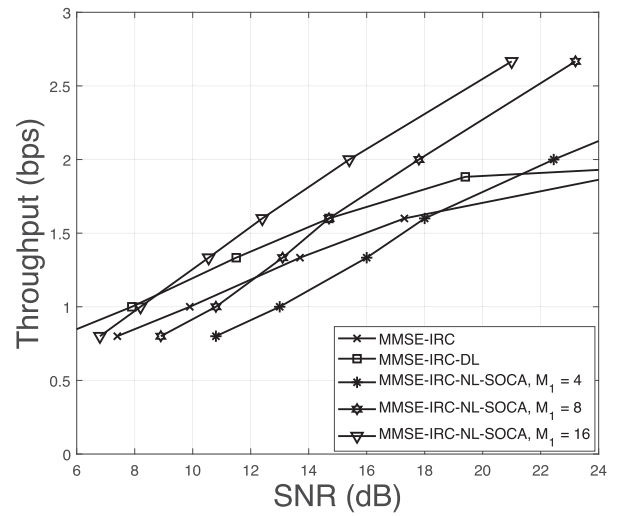
FIGURE 14. Throughput as a function of the SNR where a BLER of 10^{-1} is achieved, for the case of N_r = 4 RAs, N_u = 4 user TA, N_i = 1 interfering user TA, K' = 2048 information bits, L_{\max} = 4 slicing value, SIR = 10 dB, BG = 2, N_c = 64 subcarriers, when using 16-QAM modulation for communication over a frequency selective fading channel with L = 4 channel taps. For the NL-SOCA tree search in the case of the MMSE-IRC-NL-SOCA scheme, the number of child nodes created in each layer is M = [M_1 \ 1 \ 1 \ 1] and the number of surviving child nodes in each layer is K = [M_1 \ M_1 \ M_1 \ M_1] , where M_1 = 4, 8 and 16 are considered. The number of outer iterations performed between the NL-SOCA detector and LDPC decoder is I_{\text{outer}} = 4 .
