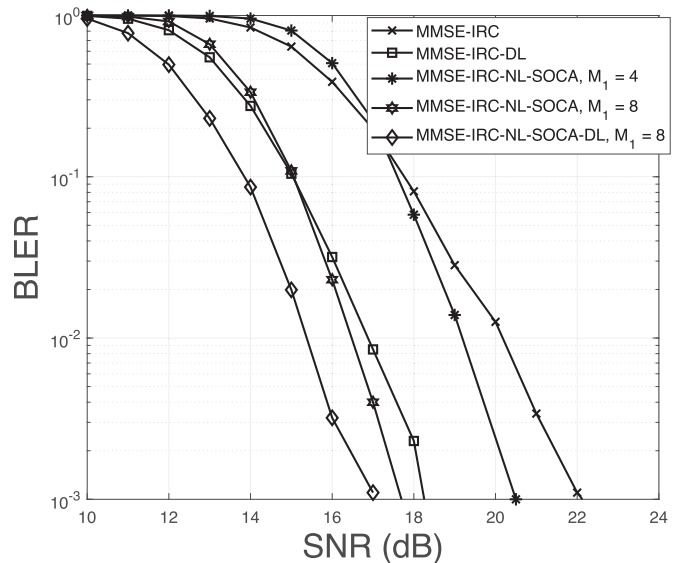
FIGURE 11. BLER performance as a function of SNR for various schemes, for the case of N_r = 4 RAs, N_u = 4 user TAs, N_i = 1 interfering user TA, K' = 2048 information bits, L_{max} = 4 slicing value, coding rate R = 1/3 , SIR = 0 dB, BG = 2, N_c = 64 subcarriers, when using 16-QAM modulation for communication over a frequency selective fading channel with L = 4 channel taps. For the NL-SOCA tree search in the case of the MMSE-IRC-NL-SOCA and MMSE-IRC-NL-SOCA-DL schemes, the number of child nodes created in each layer is M = [M_1 \ 1 \ 1 \ 1] and the number of surviving child nodes in each layer is K = [M_1 \ M_1 \ M_1 \ M_1] , where M_1 = 4 and 8 are considered. The number of outer iterations performed between the NL-SOCA detector and LDPC decoder is I_{outer} = 4 .
