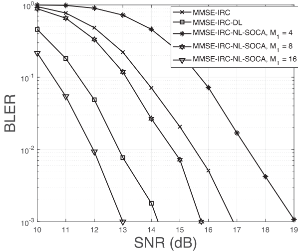
FIGURE 12. BLER performance as a function of SNR for various schemes, for the case of N_r = 4 RAs, N_u = 4 user TAs, N_i = 1 interfering user TA, K' = 2048 information bits, L_{\max} = 4 clipping value, coding rate R = 1/3 , SIR = 10 dB, BG = 2, N_c = 64 subcarriers, when using 16-QAM modulation for communication over a frequency selective fading channel with L = 4 channel taps. For the NL-SOCA tree search in the case of the MMSE-IRC-NL-SOCA scheme, the number of child nodes created in each layer is M = [M_1 \ 1 \ 1 \ 1] and the number of surviving child nodes in each layer is K = [M_1 \ M_1 \ M_1 \ M_1] , where M_1 = 4, 8 and 16 are considered. The number of outer iterations performed between the NL-SOCA detector and LDPC decoder is I_{\text{outer}} = 4 .
