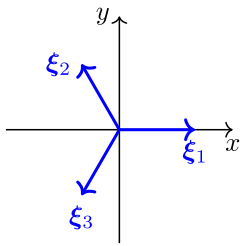
FIGURE 2. Hexagonal box-spline vectors.
