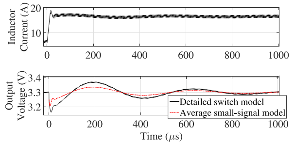
FIGURE 26. Similar operating condition as in Fig. 25, except with f_c = f_{sw}/5 .
