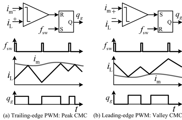
FIGURE 4. Two PWM current mode control techniques.
