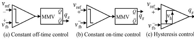
FIGURE 14. Voltage-ripple-based variable frequency control methods [69].
