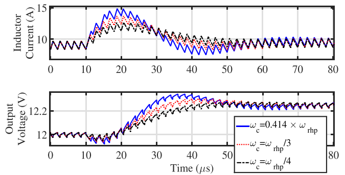
FIGURE 31. Transient response of a CMC boost converter for a step change in v_{ref} from 12 to 12.25 V with v_{in} = 8 V and R = 2 \Omega using different \omega_c values.
