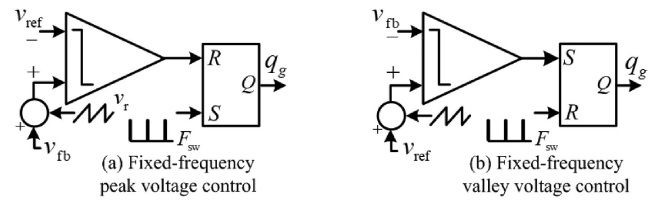
FIGURE 15. Voltage-ripple-based fixed-frequency control methods [69].
