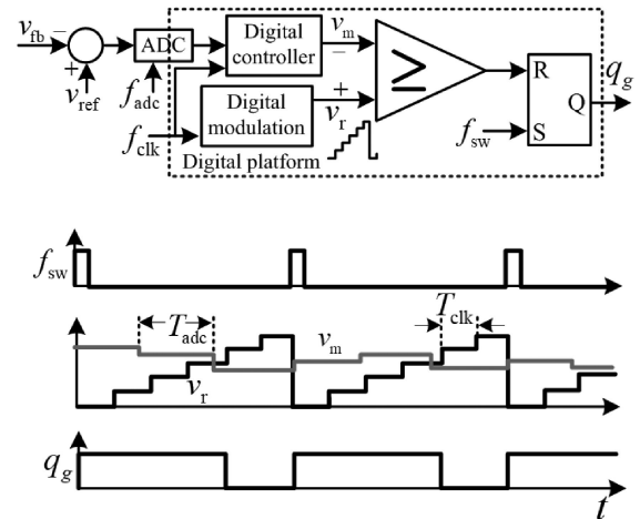
FIGURE 6. Fixed-frequency (trailing-edge) digital pulse width modulation.
