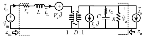
FIGURE 22. Small signal equivalent circuit of a synchronous boost converter.
