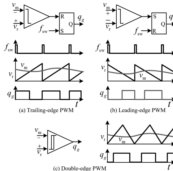
FIGURE 3. Three PWM carriers for dc-dc converters.
