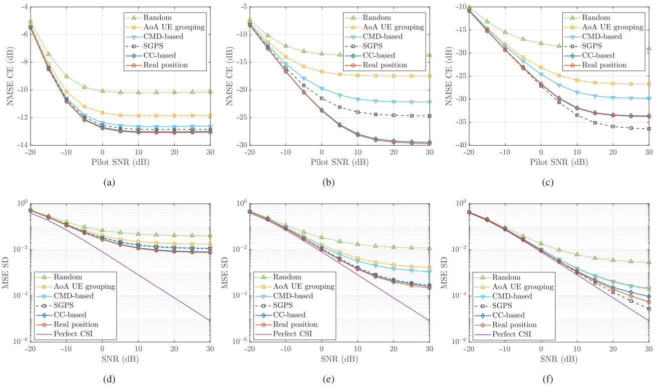
FIGURE 8. NMSE CE and MSE SD versus the SNR for distinct pilot reuse factors, N/\tau = \{16, 8, 4\} , respectively, and for different pilot assignment algorithms. (a) and (d) \tau = 32 , (b) and (e) \tau = 64 , and (c) and (f) \tau = 128 .
