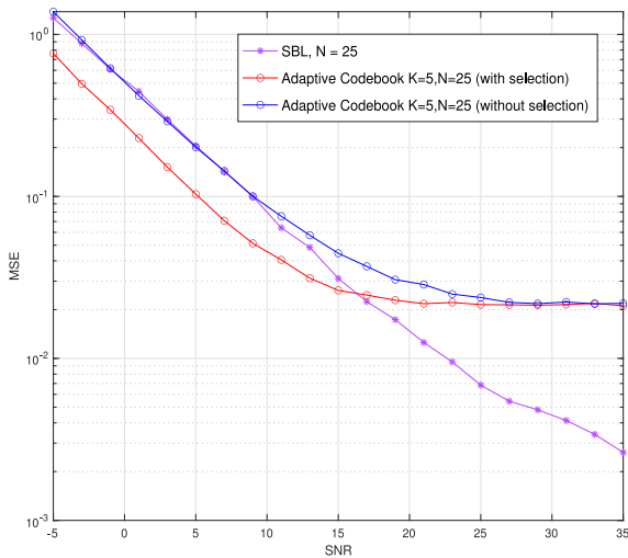
FIGURE 6. Comparison of MSE performance of the codebook-based and SBL-based channel estimation, when N_t = 8 and N_r = 8 .
