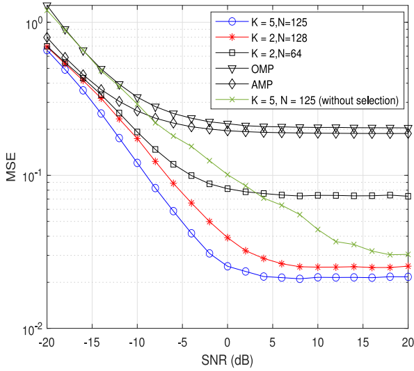
FIGURE 5. MSE performance of channel estimation with different K and N values.
