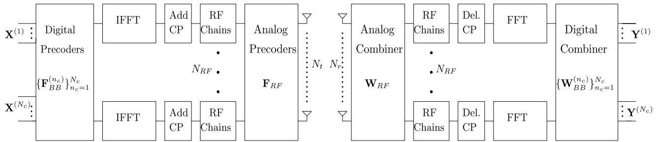
FIGURE 1. Block diagram of mmWave OFDM system.
