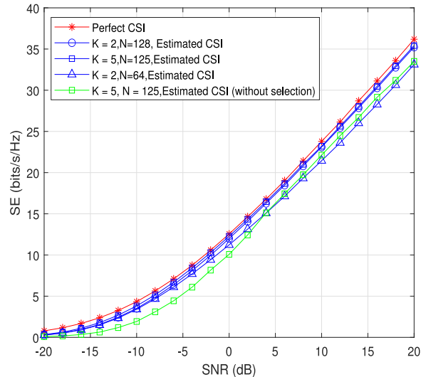
FIGURE 7. Achievable rates of the OFDM systems with respectively the proposed channel estimation and the conventional codebook-based channel estimation.
