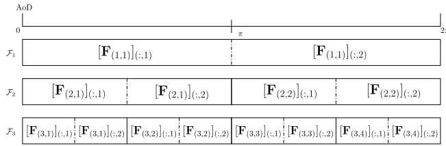
FIGURE 2. Multi-resolution codebook structure with S = 3 stages and each subset having K = 2 codewords.
