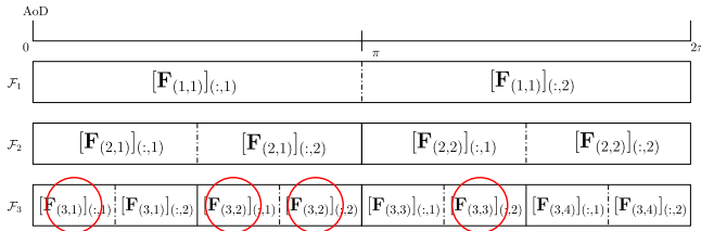
FIGURE 4. Example for illustrating the proposed channel estimation scheme.
