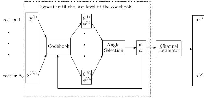
FIGURE 3. Block diagram of our proposed channel estimation technique.
