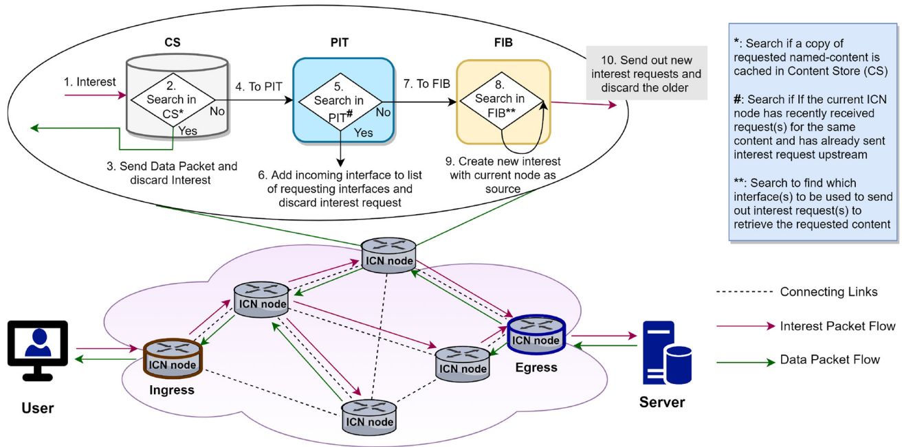
FIGURE 2. Flow of interest packet and data packets in CCN [50].
