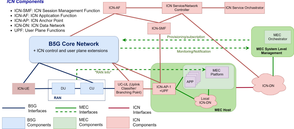
FIGURE 6. Architectural integration of MEC and ICN in 5G and beyond networks [1], [100], [142].
