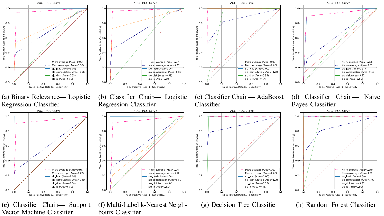
FIGURE 3. AUC-ROC plots depicting the learning of the various machine learning classifiers on individual class labels, as well as the micro and macro averaged performance on the entire set.
