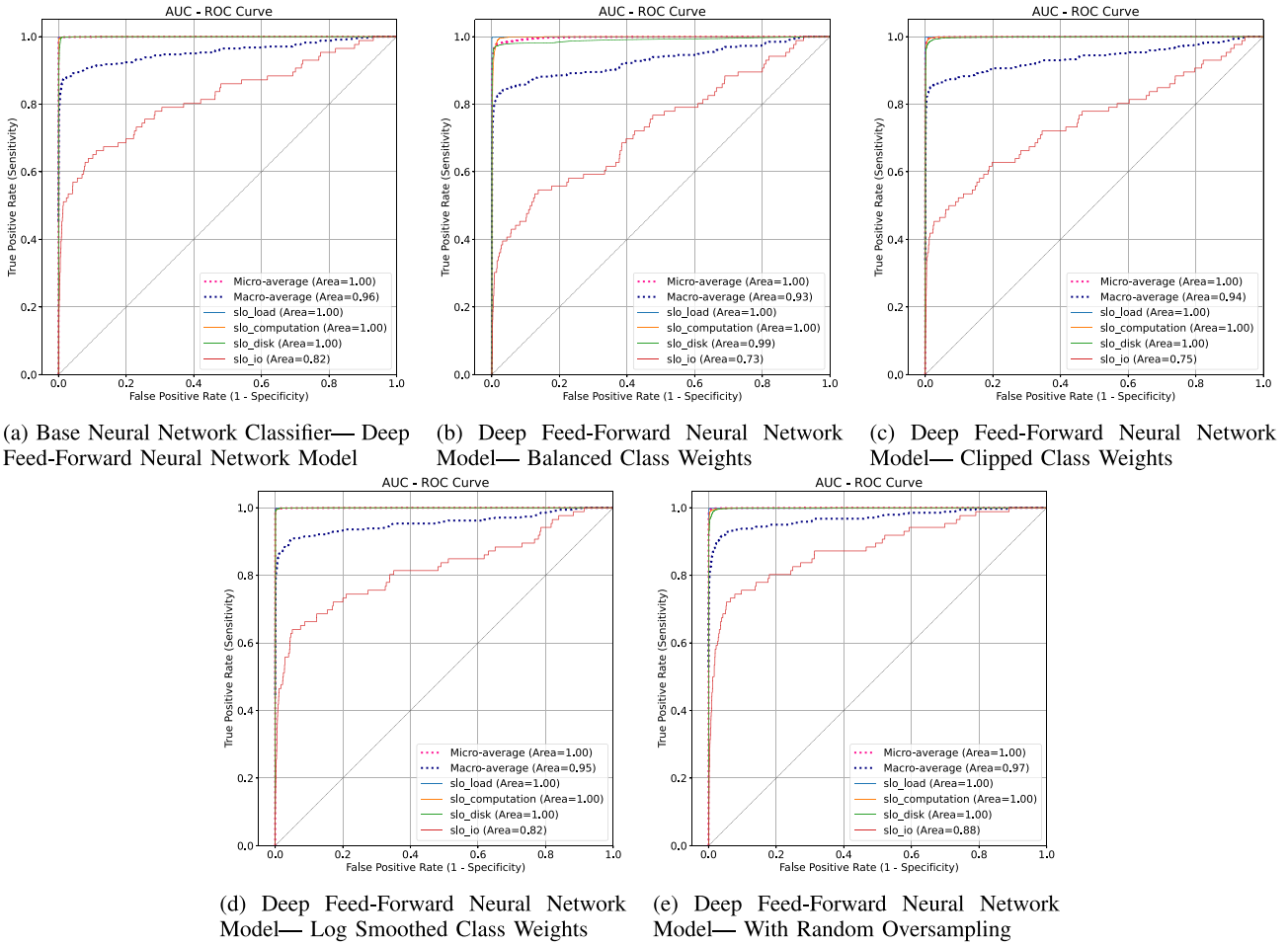
FIGURE 6. AUC-ROC plots depicting the learning of the various deep neural network classifiers on individual class labels, as well as the micro and macro averaged performance on the entire set.
