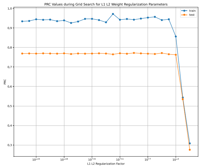
FIGURE 13. Grid search for L1 L2 weight regularization on the deep FFNN architecture used for the oversampled training set.
