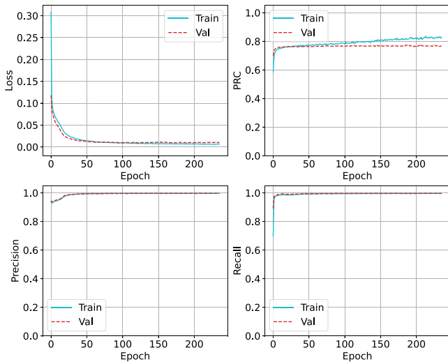
FIGURE 10. Learning Curves depicting training and validation performance for Deep Feed-Forward Neural Network Model—Log Smoothed Class Weights.
