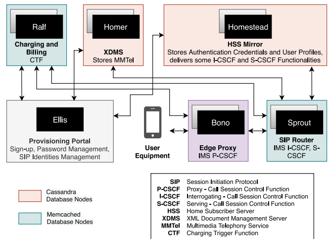
FIGURE 2. Clearwater vIMS architecture, depicting the various VNFCs and their high-level functionalities.
