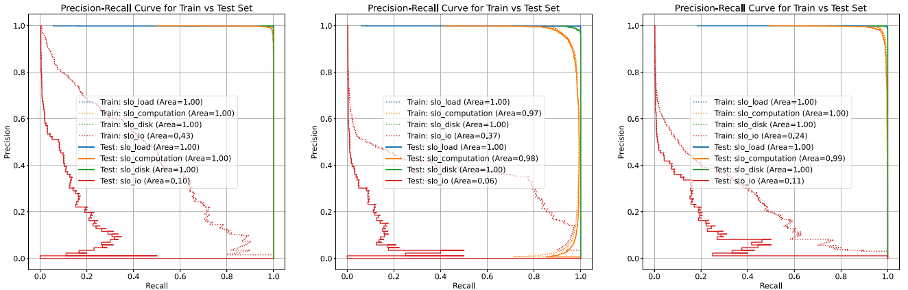
(a) Base Neural Network Classifier—Deep Feed-Forward Neural Network Model (b) Deep Feed-Forward Neural Network Model—Balanced Class Weights (c) Deep Feed-Forward Neural Network Model—Clipped Class Weights
