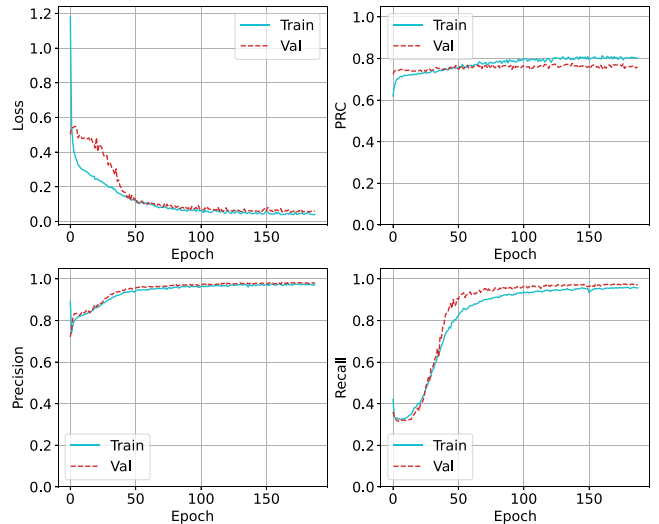
FIGURE 8. Learning Curves depicting training and validation performance for Deep Feed-Forward Neural Network Model—Balanced Class Weights.
