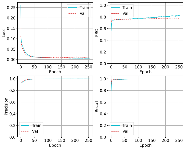
FIGURE 7. Learning Curves depicting training and validation performance for Base Neural Network Classifier—Deep Feed-Forward Neural Network Model.
