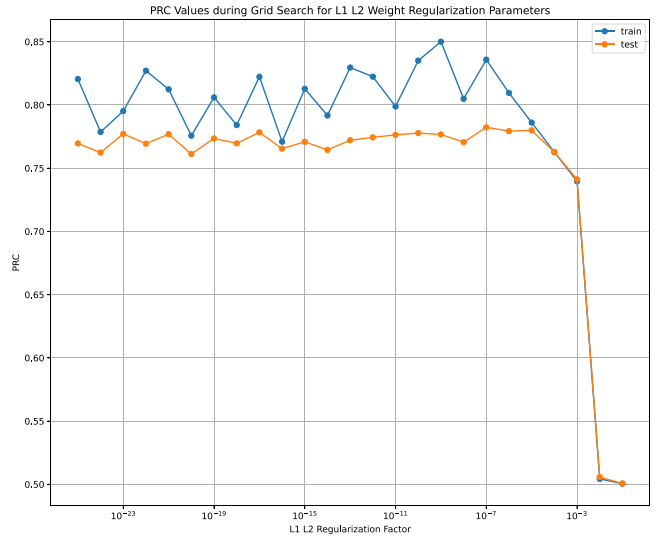
FIGURE 12. Grid search for L1 L2 weight regularization on the deep FFNN architecture.
