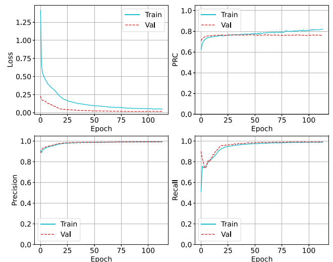
FIGURE 9. Learning Curves depicting training and validation performance for Deep Feed-Forward Neural Network Model—Clipped Class Weights.
