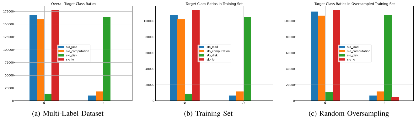
FIGURE 4. Overall distribution of the 4 SLO class labels. The training set contains a positive distribution of 5.64%, 10.05%, 92.16%, 0.23% respectively on the four SLO classes.
