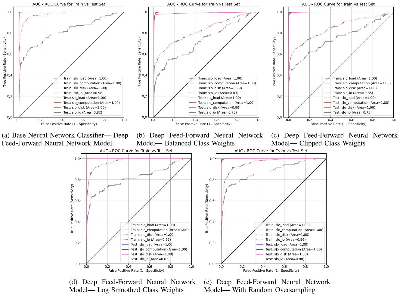
FIGURE 14. AUC-ROC plots depicting the performance of the various deep neural network classifiers on individual class labels on the Train vs Test set, signifying the degree of overfitting.
