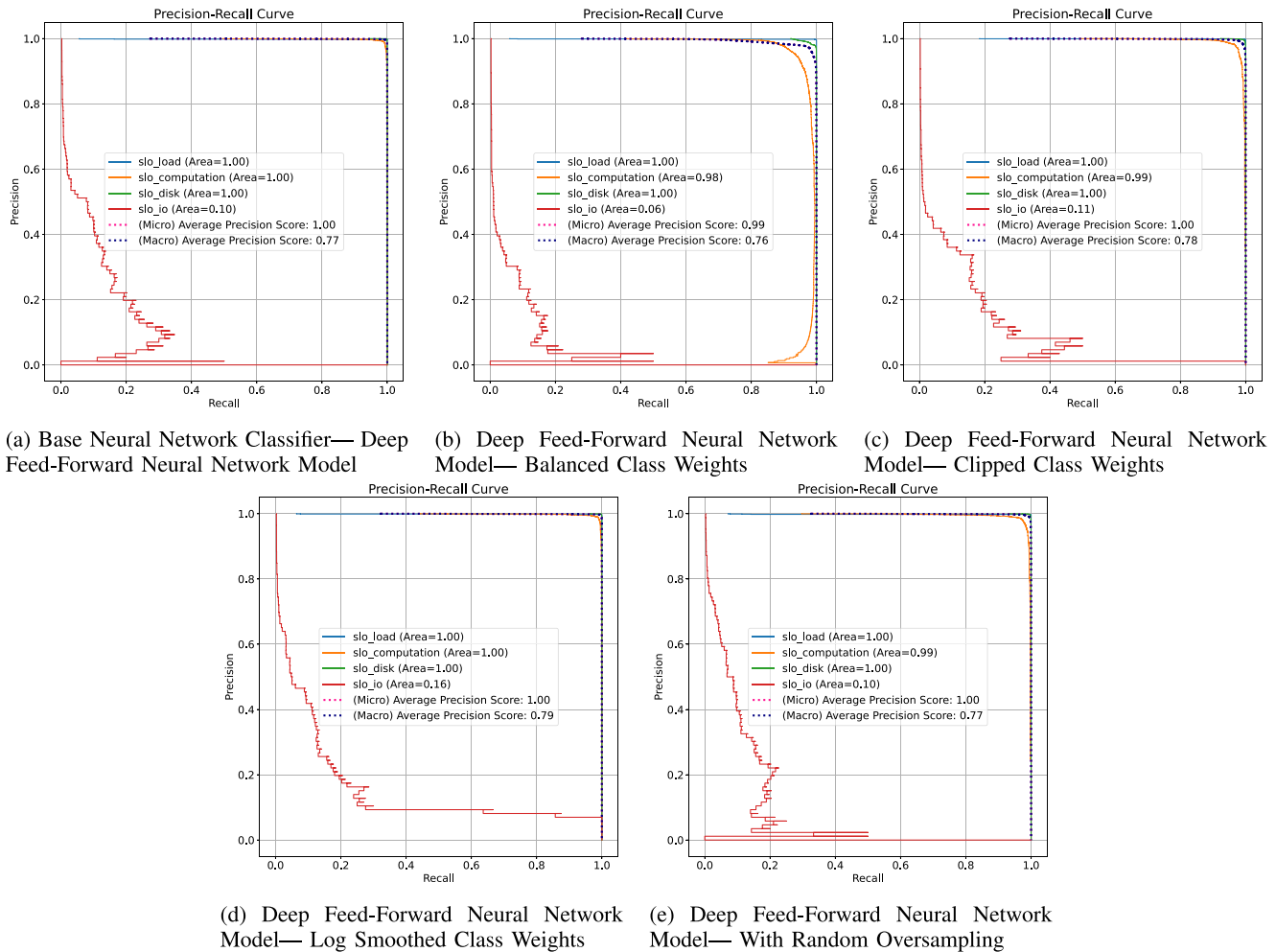
FIGURE 5. AUC-PRC plots depicting the learning and precision-recall trade-off of the various deep neural network classifiers on individual class labels, as well as the micro and macro averaged performance on the entire set.
