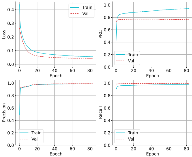
FIGURE 11. Learning Curves depicting training and validation performance for Deep Feed-Forward Neural Network Model—With Random Oversampling.
