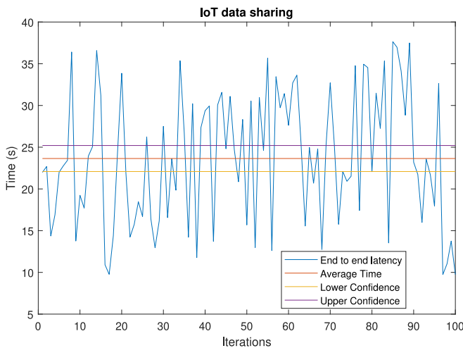
FIGURE 21. End to end latency of IoT data sharing.
