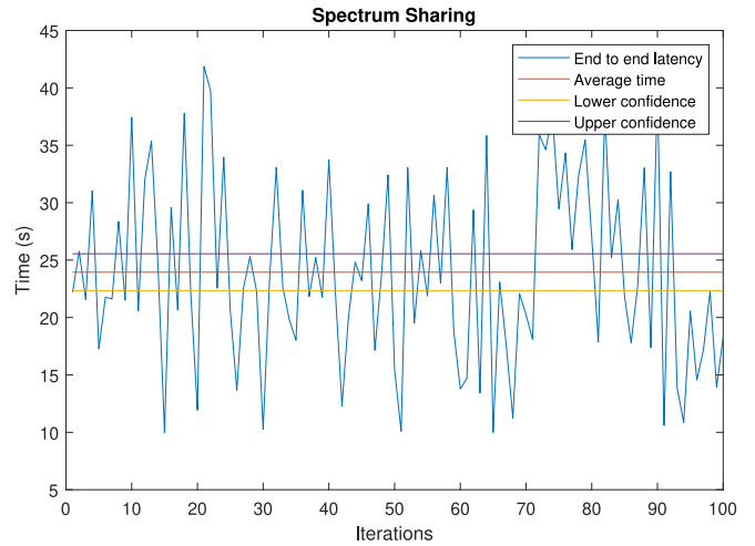
FIGURE 19. End to end latency of spectrum sharing.
