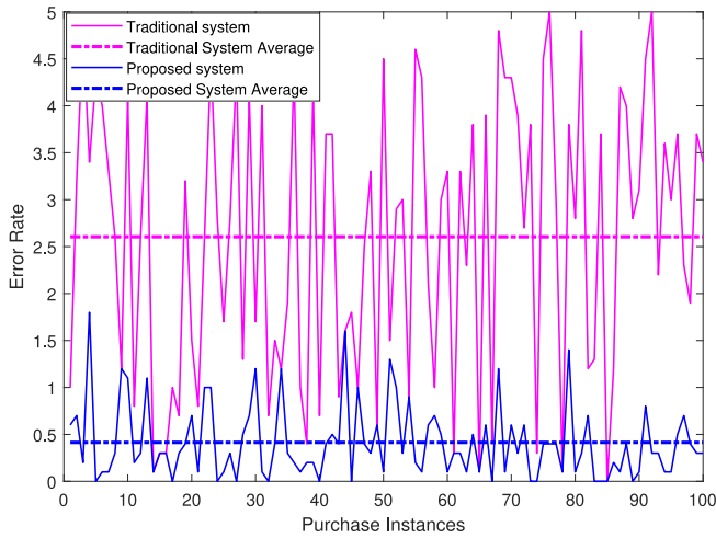
FIGURE 12. Error rate vs purchase instances.
