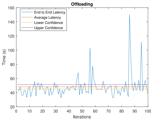
FIGURE 18. End to end latency of offloading process.
