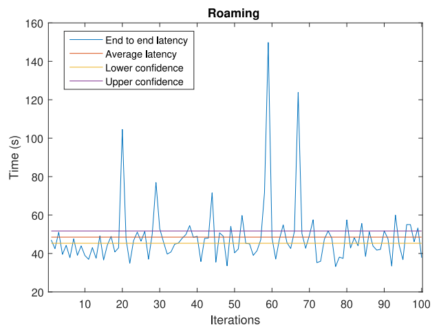
FIGURE 17. End to end latency of roaming process.
