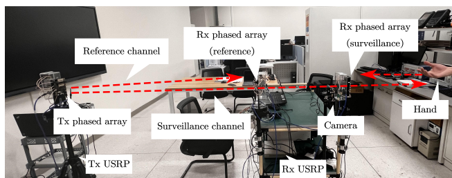
FIGURE 6. Facilities and scenario of experiment.
