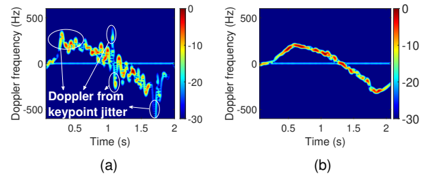
FIGURE 4. Comparison of simulated spectrograms via CASTER. (a) before one-euro filter smoothing; (b) after one-euro filter smoothing.
