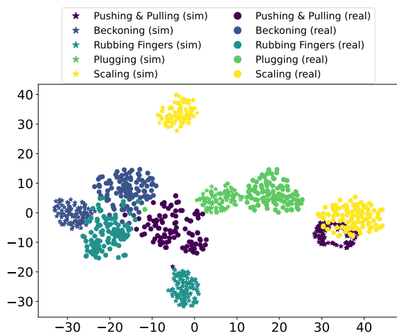
FIGURE 10. t-SNE visualization for the feature spaces of simulation and experimental datasets. Five gesture categories are distinguished by different colors, with simulation sample features denoted by star shapes and experimental sample features represented by solid circle shapes.
