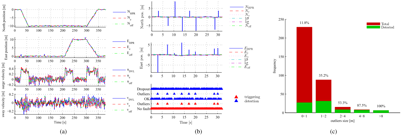
Fig. 5. (a) Measurements and state estimation when the ROV was moving along a triangular path. (b) Measurements and state estimation using HPR even during dropout. (c) State estimation after detection and removal of outliers.
