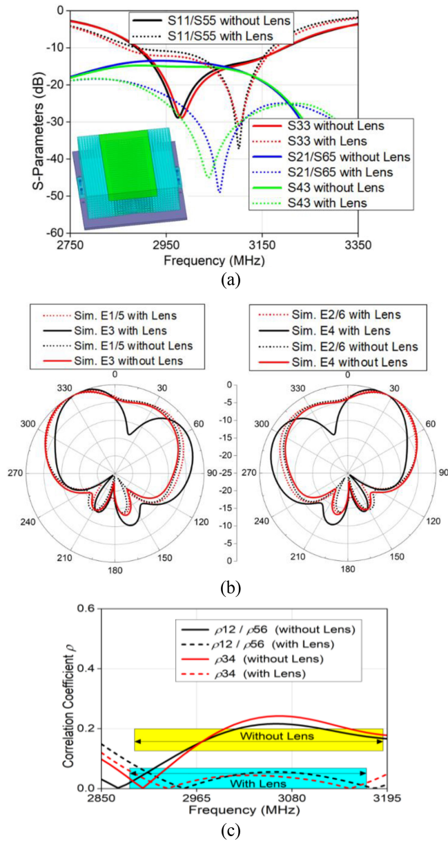
FIGURE 14. Simulated results of 6-element MIMO antenna with and without lens. (a) S-parameters. (b) Normalized radiation pattern E1/ E3/ E5 and E2/ E4/ E6 in the xoy-plane. (c) Correlation coefficient.
