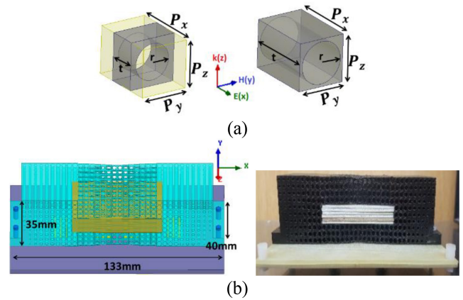
FIGURE 7. (a) Dielectric unit cell for effective permittivity of 1.25 and 1.63, where P_x = 5 mm, P_y = P_z = 3.5 mm. (b) Geometry of the lens loaded 2-element H-plane decoupled MIMO antenna.
