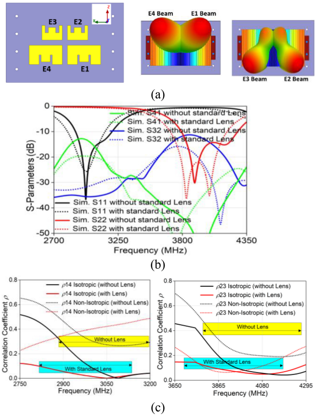
FIGURE 15. (a) 4-element Multiband MIMO antenna with and without lens. (b) S-parameters. (c) Correlation Coefficient.
