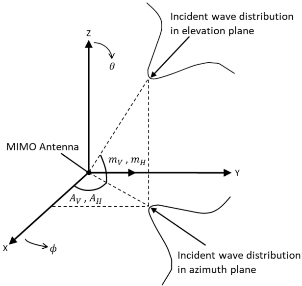
FIGURE 2. Gaussian distribution model of incoming radio waves in a multipath propagation environment.
