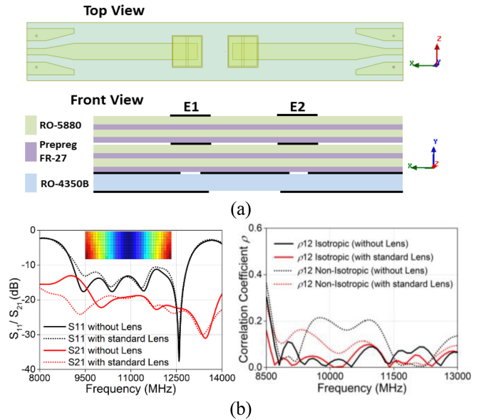
FIGURE 17. (a) 2-element Stacked MIMO antenna with and without standard lens. (b) S-parameters and Correlation Coefficient.
