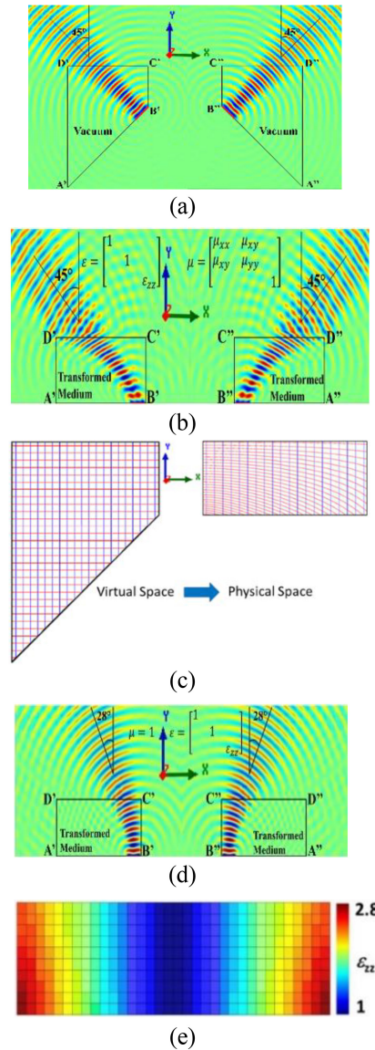
FIGURE 5. Space mapping illustration. (a) Air-filled initial virtual space. (b) Calculated transformed ideal anisotropic lens. (c) QCTE mapping from virtual space to physical space. (d) Calculated simplified quasi-isotropic lens. (e) Permittivity ( \epsilon_{zz} ) profile of simplified quasi-isotropic lens.
