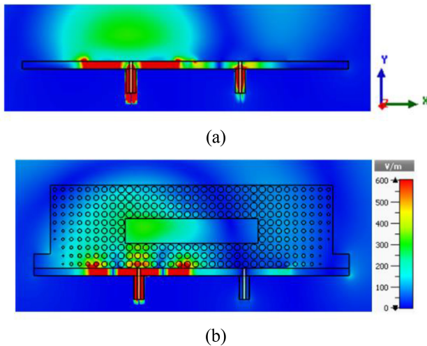
FIGURE 11. E-field distribution of 2-element H-plane coupled MIMO antenna. (a) Without lens. (b) With lens.
