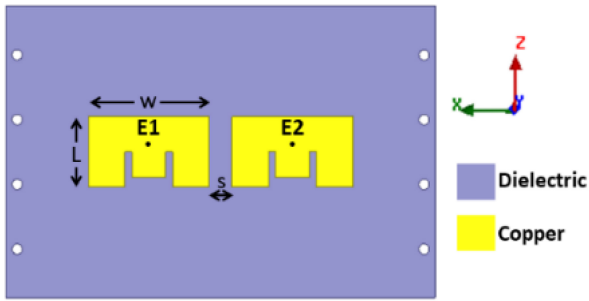
FIGURE 3. H-plane coupled 2-element E-patch MIMO antenna.
