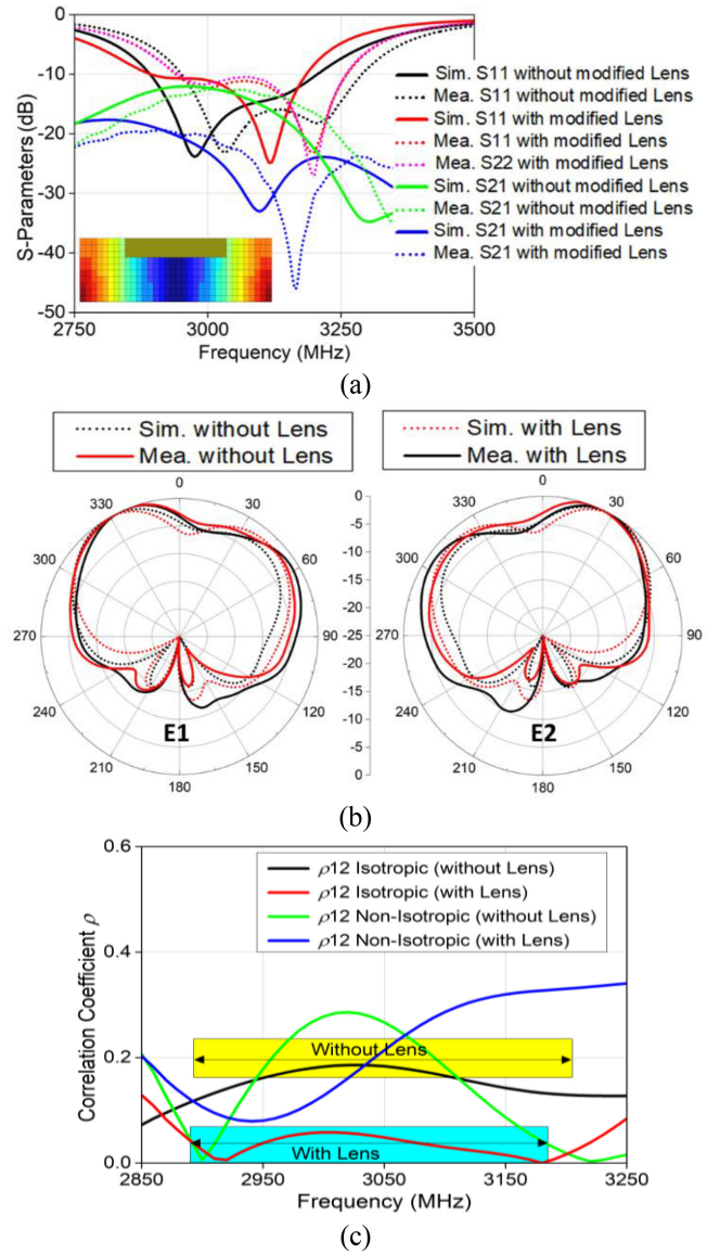
FIGURE 13. Simulated and measured results of 2-elements E-plane coupled MIMO antenna with and without lens. (a) S-parameters. (b) Normalized radiation pattern E1 and E2 in the xoy -plane. (c) Correlation coefficient.
