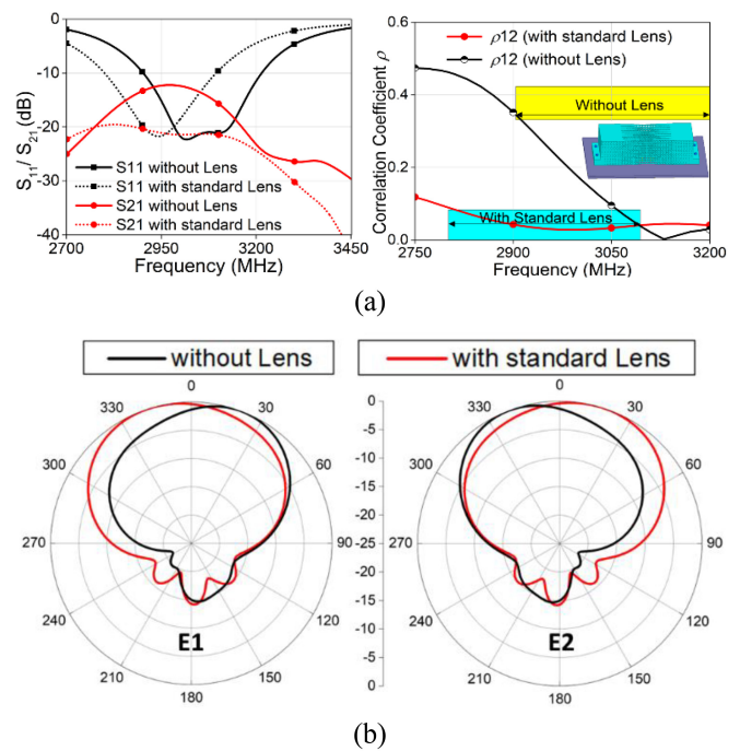
FIGURE 8. Simulated results of 2-elements MIMO antenna with and without reduced unit cell size based PLA standard lens. (a) S-parameters and Correlation Coefficient. (b) Normalized radiation pattern E1 and E2 in the xoy-plane at 3 GHz.
