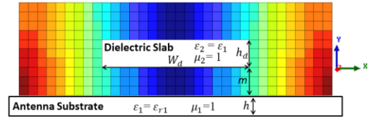
FIGURE 6. Schematic of the modified GID lens loaded E-patch MIMO antenna elements.
