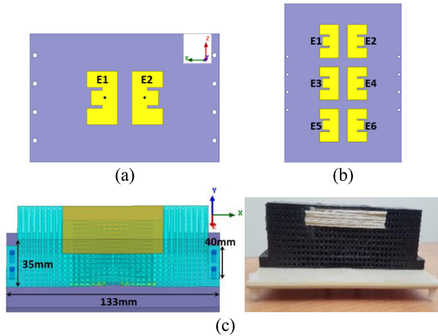
FIGURE 12. (a) E-plane coupled 2-element E-patch MIMO antenna. (b) E-plane coupled 6-element E-patch MIMO antenna. (c) Geometry of the GID lens loaded 2-element MIMO antenna.
