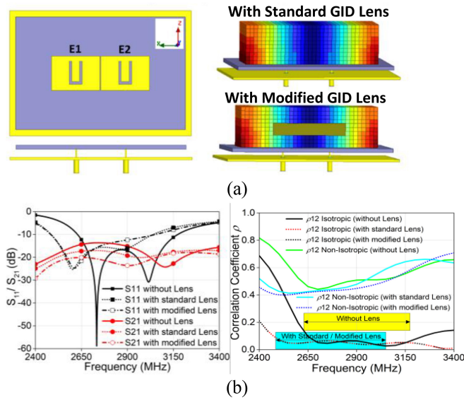
FIGURE 16. (a) 2-element U-slot MIMO antenna with and without lens. (b) S-parameters and Correlation Coefficient.
