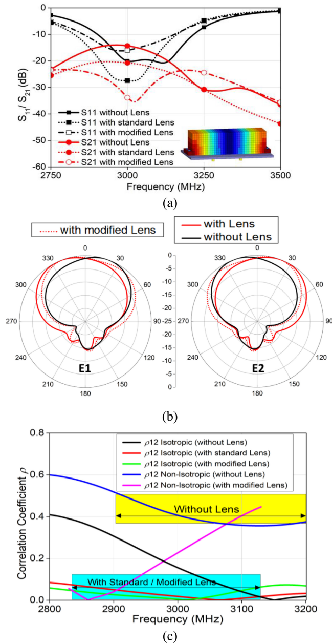
FIGURE 4. Simulated results of 2-elements MIMO antenna with and without lens. (a) S -parameters. (b) Normalized radiation pattern E1 and E2 in the xoy -plane at 3 GHz. (c) Correlation coefficient.
