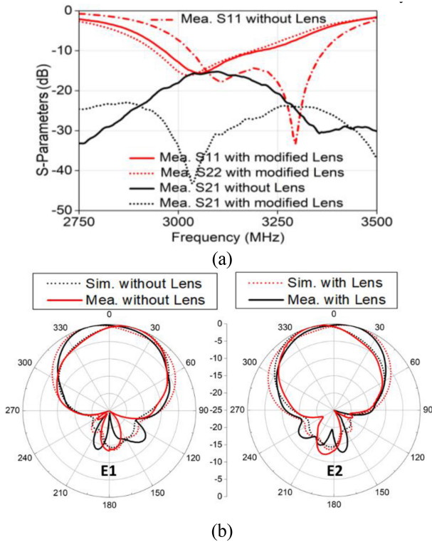
FIGURE 10. Simulated and measured results of 2-element H-plane coupled MIMO antenna with and without lens. (a) S-parameters. (b) Normalized radiation pattern E1 and E2 in the xoy -plane.
