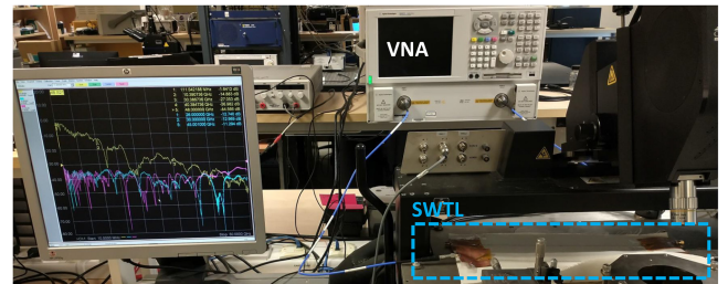
FIGURE 13. The mmWave measurement setup of the shielded SWTL.
