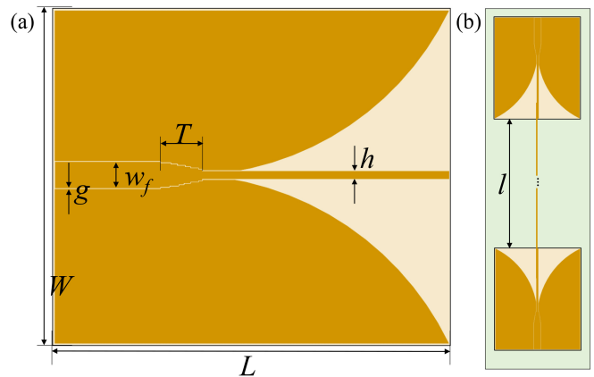
FIGURE 2. Layout and dimensions of the proposed SWTL: (a) CPW surface wave launcher; (b) the SWTL with the transmit and receive launchers; dimensions in mm: L = 61 , W = 50.5 , t = 6.5 , w_f = 4.5 , g = 0.15 , h = 1.2 .
