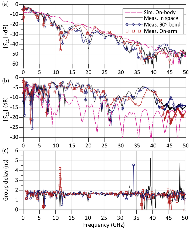
FIGURE 14. Simulated and measured mmWave transmission properties of the SWTL: (a) forward transmission; (b) reflection coefficient; (c) group delay.
