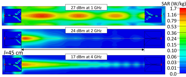
FIGURE 3. Simulated SAR across an unshielded textile SWTL with l = 45 cm at different frequencies over a uniform multi-layered tissue model; the input power level is the maximum which satisfies the 1.7 W/kg requirement.
