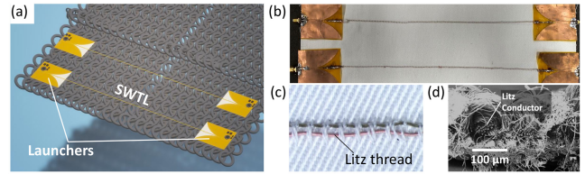
FIGURE 5. Two closely-packaged SWTLs on a polyester cotton substrate: (a) 3D mockup showing the possible component placement on the launchers; (b) photograph of the fabricated lines; (c) micrograph showing the over-stitched wire; (d) scanning electron microscope (SEM) cross-section of the Litz wire in-fabric.
