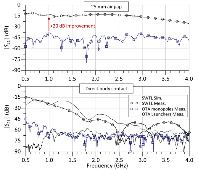
FIGURE 9. Comparison of the on-body unshielded SWTL performance relative to unconnected on-body monopoles and launchers: (a) link L_3 from Fig. 6(a) with a 5 mm air gap between the SWTL and the body; (b) link L_2 with the SWTL, launchers, and OTA antennas pressed against the body with no gap.
