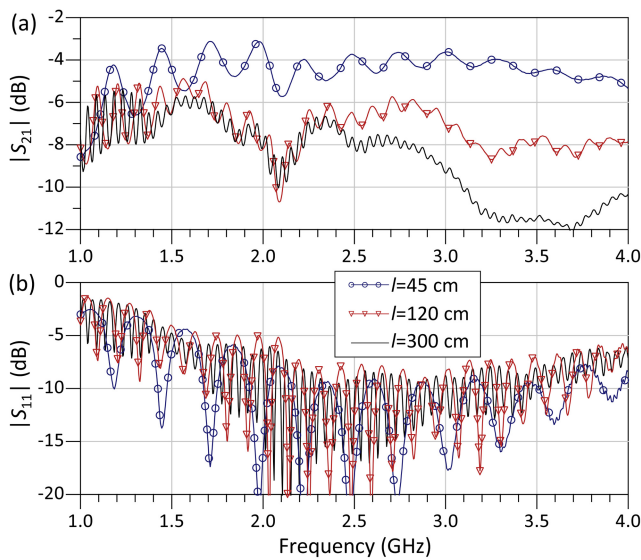
FIGURE 7. Measured s-parameters of the SWTL with different lengths in space using the setup in Fig. 6(b): (a) forward transmission; (b) reflection coefficient.
