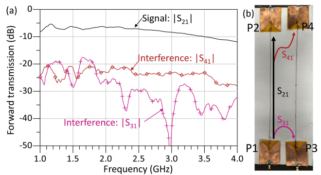
FIGURE 12. (a) Measured four-port transmission properties of the closely-coupled SWTLs; (b) the port numbering and coupling mechanism.
