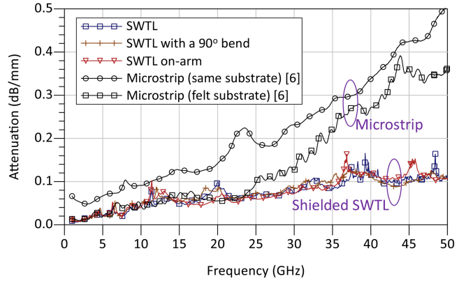
FIGURE 15. Measured attenuation of the SWTL, normalized to the line’s length, compared to the textile-based microstrip lines from [6].
