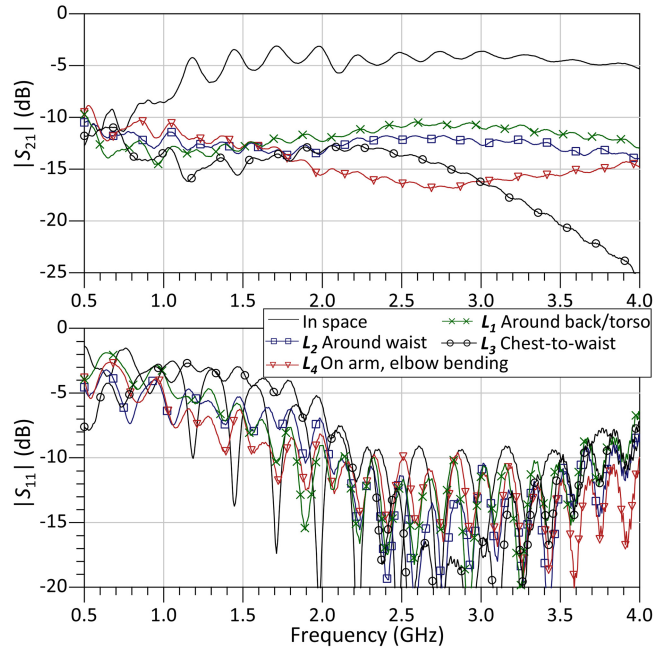
FIGURE 8. Measured s -parameters of the SWTL over for the different on-body links, whose test setups are shown in Fig. 6(a).
