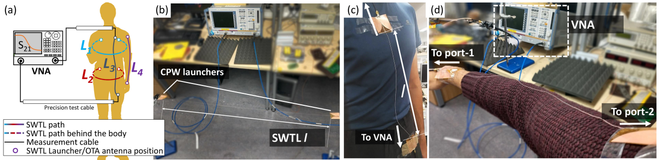
FIGURE 6. The on-body measurement setup of the SWTL: (a) positions of the on-body links investigated; (b) photograph the in-space SWTL measurement setup; (c) photograph of link L_4 ; (d) photograph of link L_3 .
