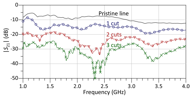
FIGURE 11. Measured forward transmission of the 45 cm-long SWTL for a different number of 10 cm-spaced gaps.
