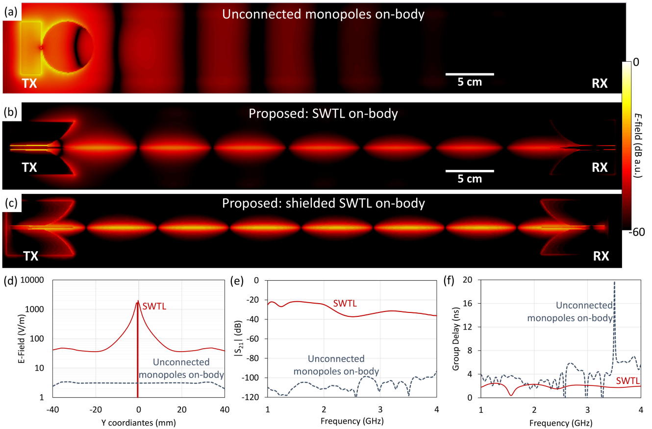
FIGURE 1. Simulated performance of an on-body SWTL compared to unconnected omnidirectional monopoles for a 45 cm link at 2 GHz: (a) E -field plot of unconnected on-body monopoles (benchmarking reference); (b) E -field plot of the proposed on-body SWTL; (c) E -field plot of the proposed on-body SWTL backed by a shielding conductive plane; (d) 1D E -field cross-section at half-way through the link, i.e., at 22 cm from the transmitter; (e) the forward transmission between the two on-body ports; (f) the group delay of the OTA link and the SWTL.
