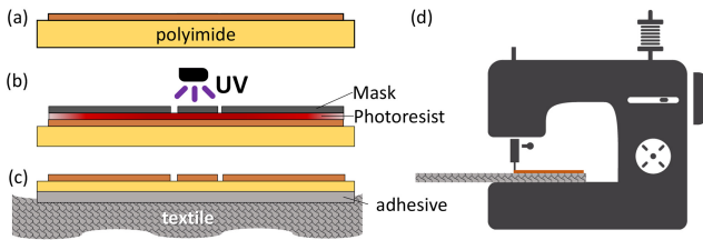
FIGURE 4. Fabrication steps of the e-textile SWTL: (a) flexible polyimide (Kapton) copper laminate; (b) photolithography of the launcher's patterns using UV exposure and chemical etching [7]; (c) attachment of the flexible polyimide-based launcher/circuit onto the textile substrate [6]; (d) over-stitching of the fabric Litz thread onto the same textile substrate [32].
