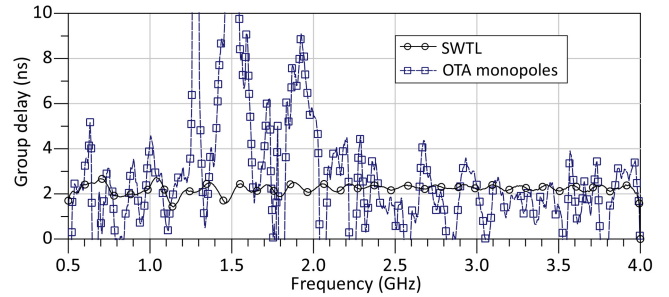
FIGURE 10. Measured group delay of the SWTL and the on-body monopoles for a chest-to-waist link, shown in Fig. 6(b).
