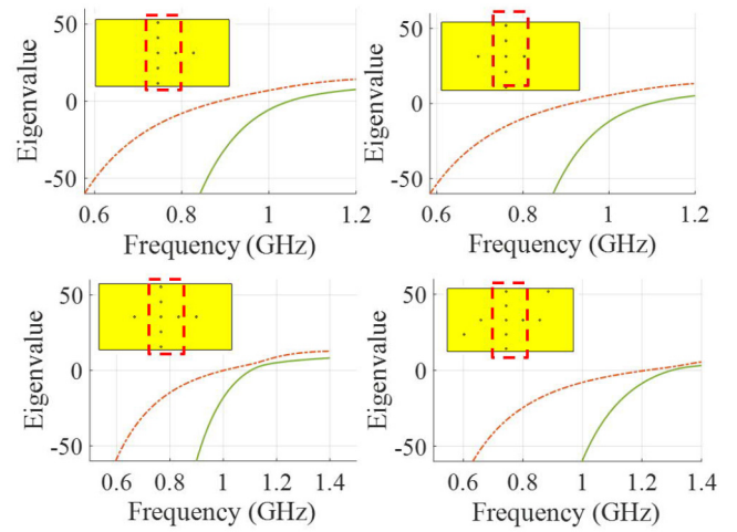
FIGURE 16. Different number of shorting pins added in random locations between the chassis and screen. The red dashed rectangle is showing the original pins we used in Fig. 1(b).
