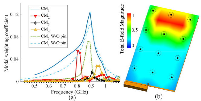
FIGURE 9. (a) Modal weighting coefficient of the modes for P_3 and, (b) electric near-field of the CM_3 mode (half-way between the screen and the PCB) after adding a shoring pin close to the single CCE.
