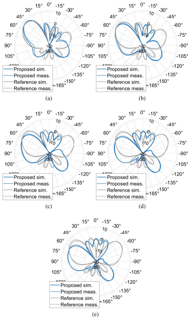
FIGURE 11. Simulated and measured realized gains of the reference and proposed array in the xz -plane when the steering angle is optimized for (a) 50^\circ , (b) 60^\circ , (c) 70^\circ , (d) 80^\circ , and (e) 90^\circ .
