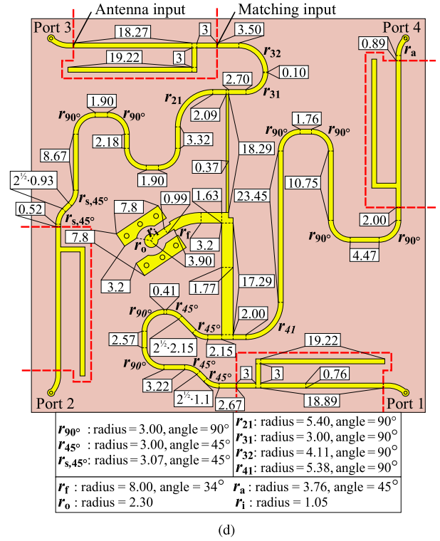
FIGURE 2. Cross-section (a) and layers (ground (b), antenna (c), and signal (d)) of the proposed antenna. All dimensions are in millimetres.
