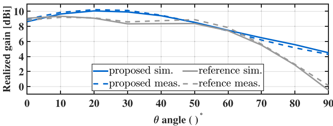
FIGURE 9. Simulated and measured realized gains of the proposed and reference antenna array as a function of the optimized steering angle.
