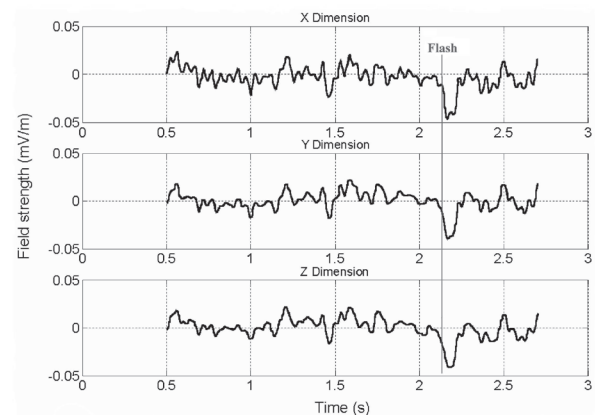
Figure 1: Measurements of a strobe flash discharge
