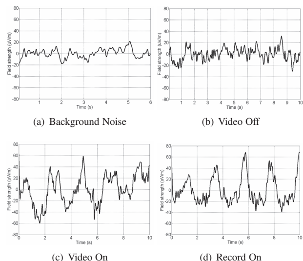
Figure 2: Amplitude measurements with the Video Camera
