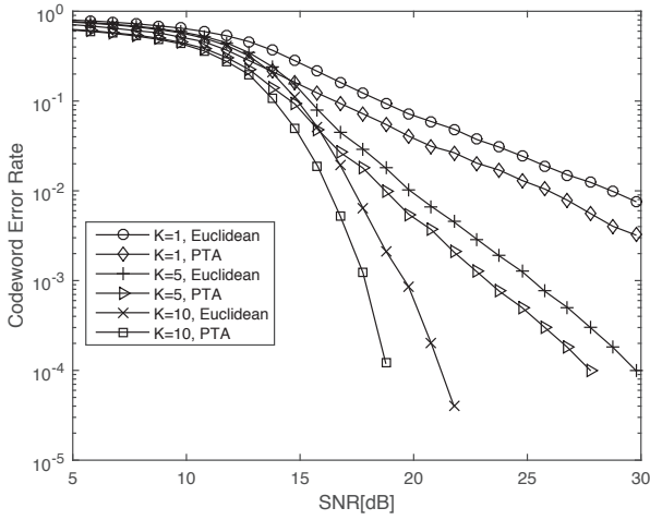
Figure 4: Comparison of soft-decision and hard-decision RS decoding for different Rician K factors, C_r = \frac{5}{15}
