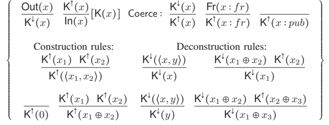
Fig. 4: Set of normal deduction rules ND_{\text{XOR}}
