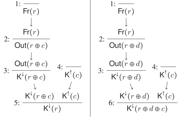
Fig. 6: Dependency graph for an instance of the example protocol and its mirror.
