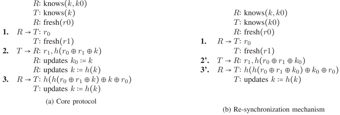
Fig. 7: Alice&Bob description of LAK'06 [46]
