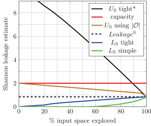
Figure 3: Shannon leakage estimates for CRIME (size 3).
