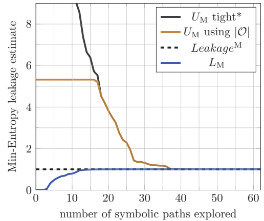
Figure 6: Estimates of CheckSecret's min-entropy leakage (guess=1000, \mathcal{D} = \{0, \dots, 10000\} , size of t=30 ).
