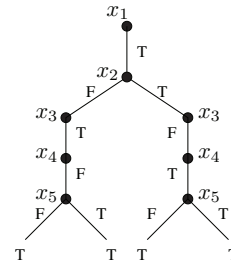
Fig. 5: Model for the QBF instance in Fig. 4.
