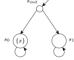
Fig. 6: Kripke structure in the proof of Theorem 6.
