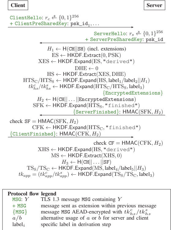
Figure 3: The TLS 1.3 draft-28 [39] PSK handshake protocol.
