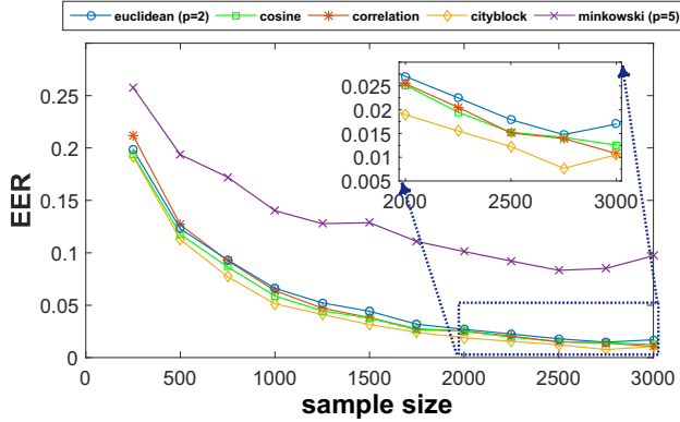
Fig. 4: Average EER according to different sample sizes using different distance metrics while users are performing Typing Task-1.
