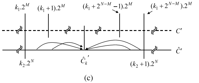
Fig. 10. Effect of bit plane discarding in watermark extraction; \lambda = 2^M and N is the number of bit plane being discarded. (a) Case 1: M > N . (b) Case 2: M = N . (c) Case 3: M < N .
