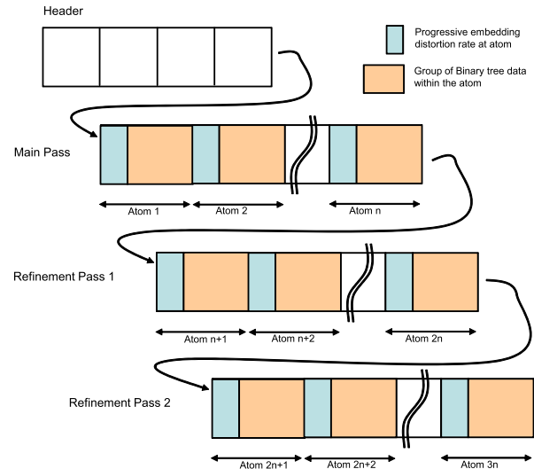
Fig. 8. Code-stream generation.
