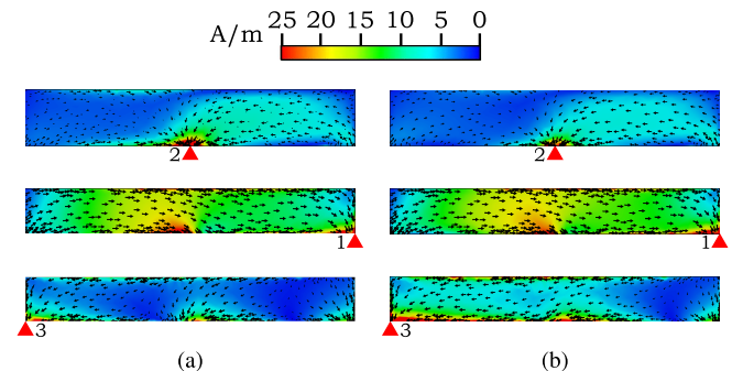
Fig. 12. Real part of the surface currents on the feeding elements of the metal-rimmed mobile antenna with (a) TARC and (b) P_{\text{rad}}/P_{\text{near}} input weights at 3.7 GHz. Locations of the discrete ports are marked with red arrows.
