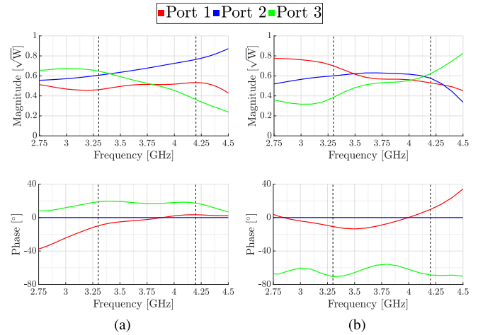
Fig. 11. Magnitude (top) and phase (bottom) of (a) TARC and (b) P_{\text{rad}}/P_{\text{near}} -optimized input weights for the metal-rimmed antenna. The n77 band is marked with a black dashed line.
