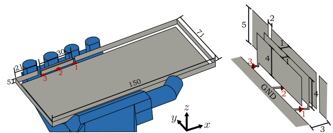
Fig. 6. Mobile antenna with a metal rim and three feeding elements. The hand model is adopted from [29].
