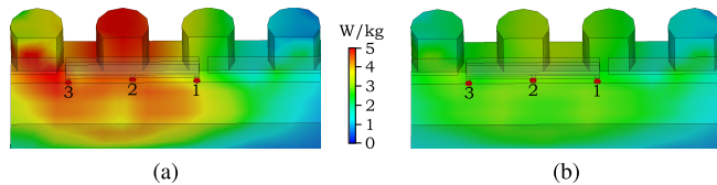
Fig. 9. 10-g SAR patterns of the metal-rimmed mobile antenna at 3.7 GHz with P_{\text{in}} = 22.4 dBm. (a) TARC and (b) P_{\text{rad}}/P_{\text{near}} optimal inputs.
