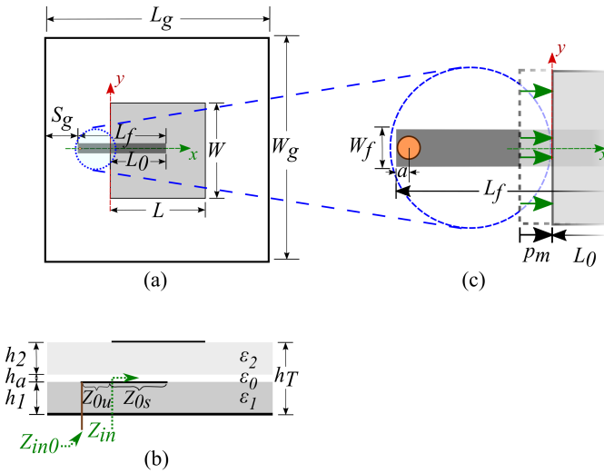
Fig. 5. Geometry and dimensions of the fabricated PC-MSPA. (a) Top view. (b) Side view, with air gap h_a between the substrates. (c) Patch movement p_m representation.
