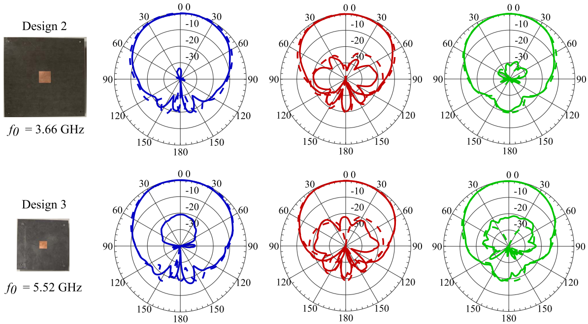
Fig. 7. Normalized co- and cross-polarized radiation patterns in the E-, D-, and H-planes (from left to right). Simulated (dashed line) and measured (solid line) radiation patterns of the design antennas' designs 2 and 3.
