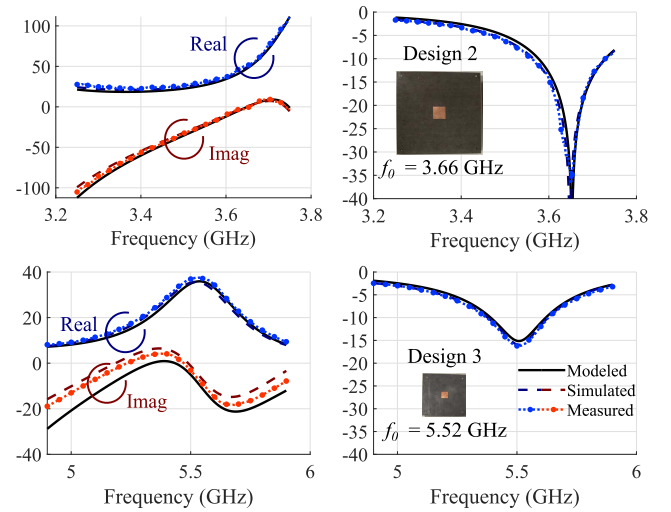
Fig. 6. Comparison between modeled, simulated, and measured impedance responses ( \Omega ) and S_{11} parameter (dB) for the fabricated antennas' designs 2 and 3.
