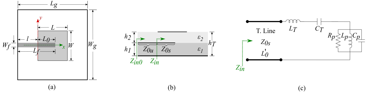
Fig. 1. Geometry and equivalent circuit model of the PC-MSPA. (a) Top view. (b) Side view. (c) Equivalent circuit model.
