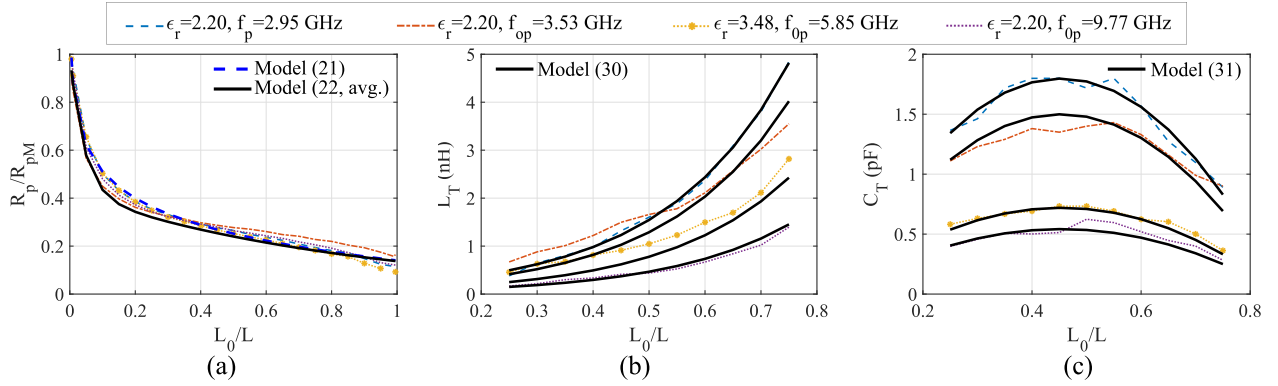
Fig. 3. Model parameters versus overlap ratio. (a) Normalized radiation resistance ( R_p/R_{pM} ). (b) Feeding inductance ( L_T ). (c) Feeding capacitance ( C_T ).
