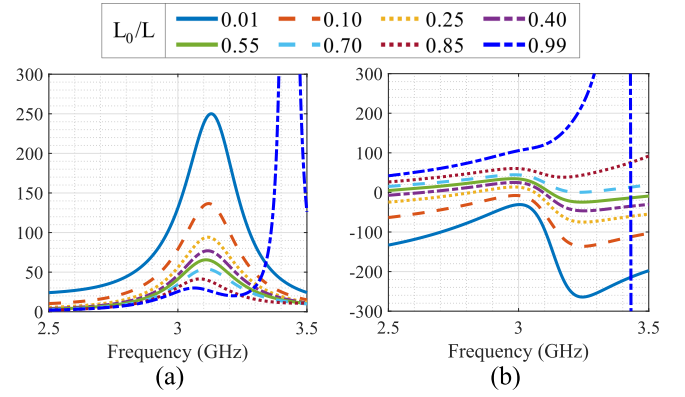
Fig. 2. Variations of impedance response of a PC-MSPA with different feed lengths. (a) Real part. (b) Imaginary part.
