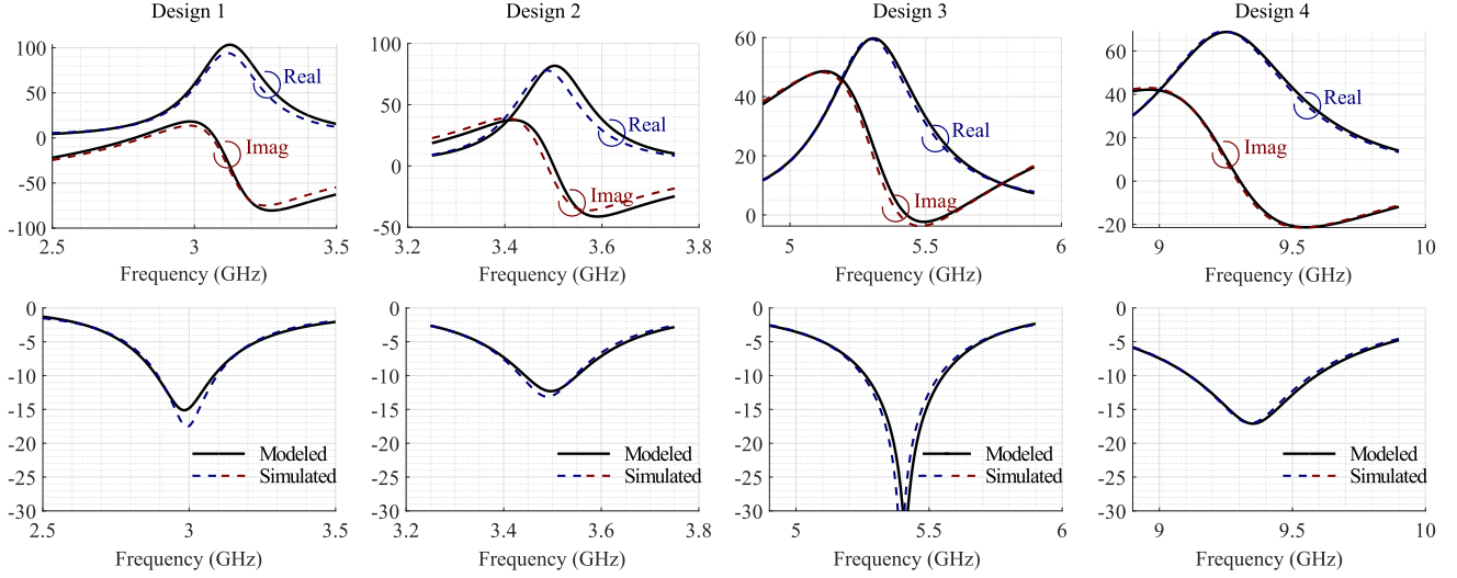
Fig. 4. Comparison between the modeled and simulated impedance responses Z_{in}(\Omega) (top row) and S_{11} (dB) (bottom row) plots.
