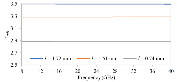
Fig. 6. Retrieved \epsilon_{\text{reff}} permittivity over frequency of the proposed unit cell with different patch lengths.
