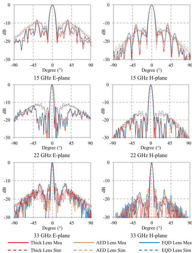
Fig. 10. Measured radiation patterns of the three lenses at 15, 22, and 33 GHz, respectively, compared with the simulated results.
