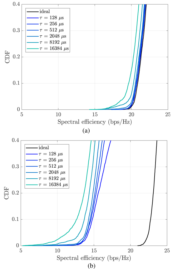
Fig. 8. Comparison of wireless propagation channels using the CDF of the spectral efficiency. To analyze the behavior over time, the calculated beamforming matrices were applied over several channel matrices delayed with \tau . (a) Measurement location marked as g_9 within Fig. 3 showing a slow-changing wireless propagation channel meaning a long coherence time. (b) Measurement location marked as g_{10} within Fig. 3 showing a fast-changing wireless propagation channel meaning a short coherence time.
