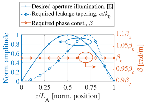
Fig. 2. Desired E -field aperture distribution, \alpha/k_0 - and \beta profiles for reduced sidelobes.
