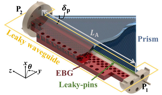
Fig. 1. Illustration of the proposed antenna. There are two main parts: leaky-wave gap waveguide (yellow) and dispersive prism (blue).
