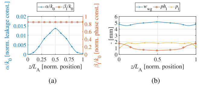
Fig. 8. Design profiles in the symmetric design. (a) Targeted leakage profile and (b) waveguide parameter profiles to synthesize the leakage profile in (a). The mapping is done at 60 GHz and the leakage is symmetric in the z -direction with respect to the center of the leaky waveguide.
