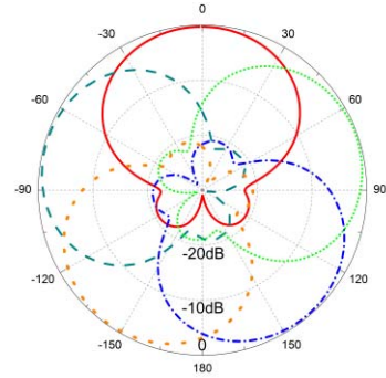
Fig. 14. Simulated switched beams at 1 pF in the H-plane.
