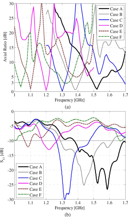
Fig. 12. Measured AR and S_{11} of the antenna. (a) Tunable AR characteristics. (b) S_{11} in the corresponding cases of (a).
