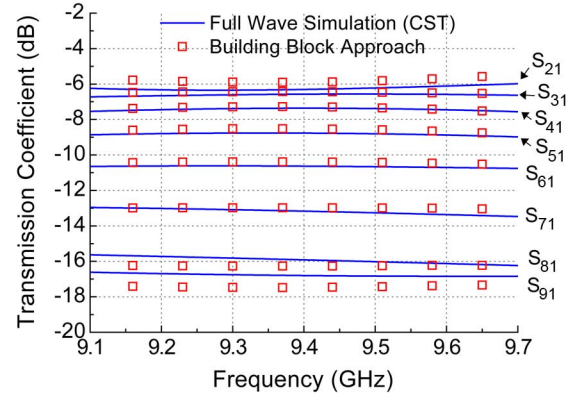
Fig. 9. Simulated amplitude characteristic of the series-fed section shown in Fig. 7 determined using a full-wave simulation tool and the building block approach.
