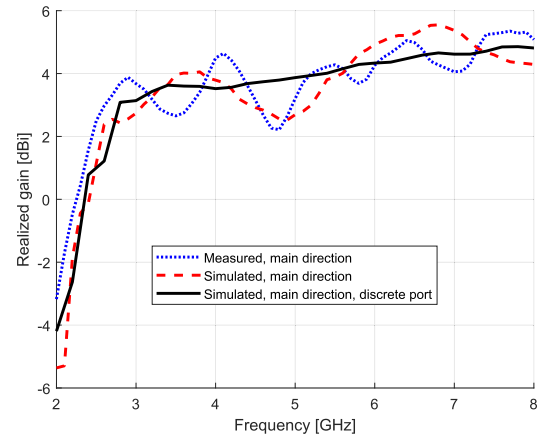
Fig. 6. Realized gain of the spiral antenna with the balun in free space.
