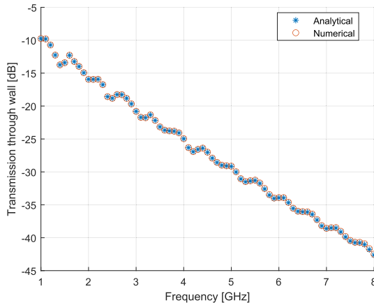
Fig. 2. Electromagnetic transmission through a bare load-bearing wall, comparison between analytical calculation and numerical simulation.
