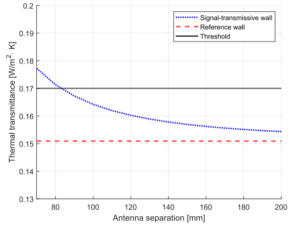
Fig. 14. Simulated thermal transmittance through the infinitely large load-bearing wall with and without the embedded spiral antenna system. The antenna separation varies from 70 to 200 mm.
