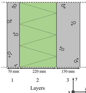
Fig. 1. Concrete sandwich panel for load-bearing wall. The panel is made of 70 mm-thick reinforced concrete (layer 1), 220 mm-thick rock wool for thermal insulation (layer 2), and 150 mm-thick reinforced concrete for structural bearing (layer 3).
