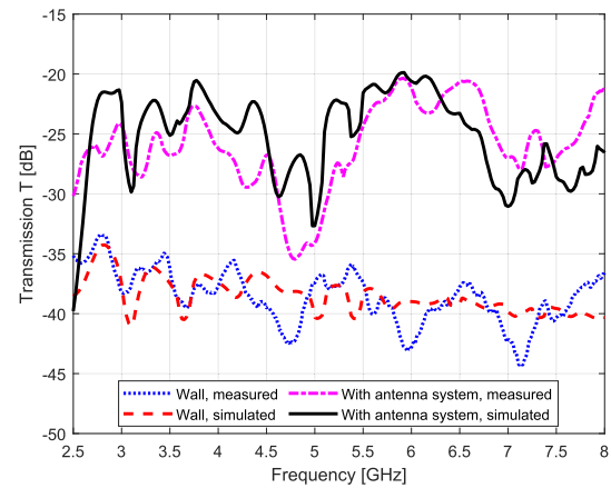
Fig. 13. Measured and simulated total electromagnetic transmission through the wall sample inside the waveguide.
