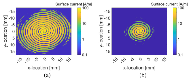
Fig. 10. Surface current of the spiral antenna at (a) 3 GHz and (b) 8 GHz.
