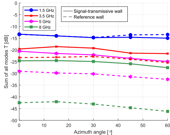
Fig. 11. Simulated transmission through the infinitely large load-bearing wall with and without the embedded spiral antenna system with a changing incident azimuth angle of a plane wave from 0^\circ to 60^\circ . The unit cell size spans 150 mm in x and y directions.
