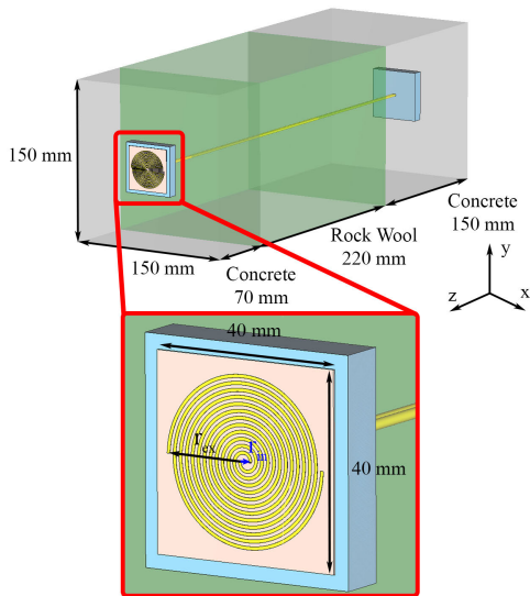
Fig. 3. Unit cell of load-bearing wall with embedded back-to-back spiral antenna system.
