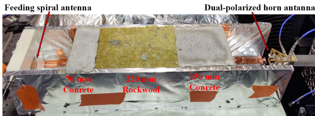
Fig. 12. Measurement setup for the electromagnetic transmission measurements. The left side is the feeding spiral antenna and on the right side, the dual-polarized horn antenna. The top-side metal is removed for the picture.
