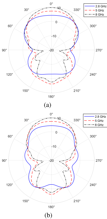
Fig. 8. Radiation pattern of spiral antenna element on top of concrete slab (a) \phi = 0^\circ and (b) \phi = 90^\circ .
