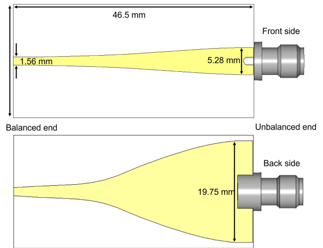
Fig. 4. Front and back view of experimentally tapered microstrip balun. Supporting legs on the top side of the connector are removed to ensure that the connector does not touch the feed line of the balun.
