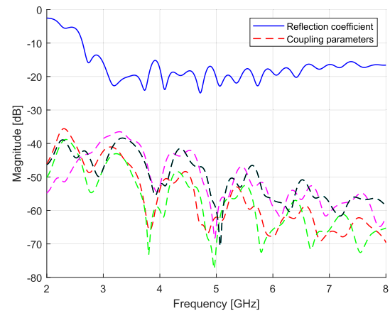
Fig. 7. Reflection coefficient and coupling parameters of spiral antenna element on top of a concrete slab.
