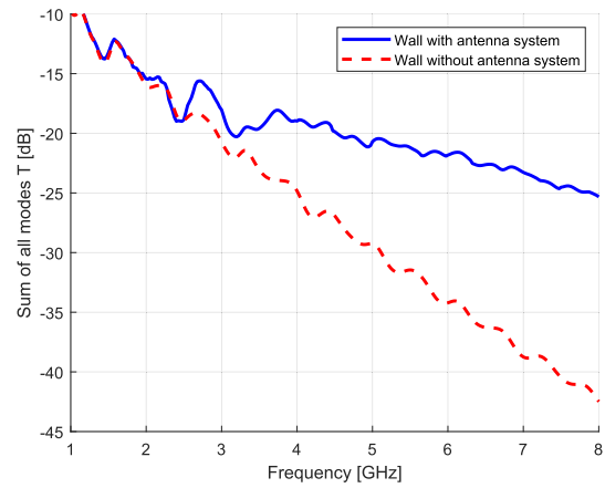
Fig. 9. Simulated transmission through the infinitely large load-bearing wall with and without the embedded spiral antenna system. The unit cell sizes in x and y directions are all 150 mm.
