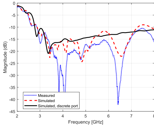
Fig. 5. Reflection coefficient of the spiral antenna in free space, measured with the balun.
