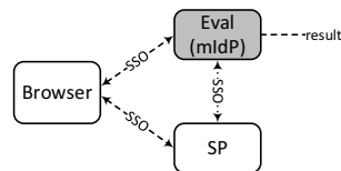
Figure 3: Attacker IdPs.
