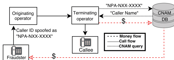
Figure 7: CNAM revenue share fraud.
