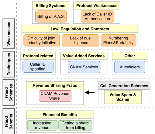
Figure 8: Taxonomy for CNAM revenue share fraud.
