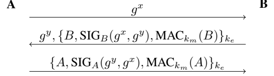
Figure 2. The SIGMA protocol with identity protection. The keys k_e and k_m are derived from g^{ab} , where k_e is used to encrypt and k_m is used to mac messages during the key exchange. Another key k_s is also derived from g^{ab} and used as session key.
