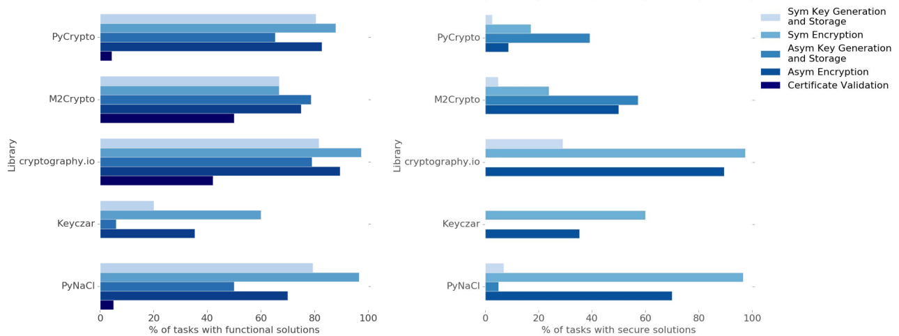
Fig. 5. Percentage of tasks with functionally correct solutions (left), and percentage of functional solutions that were rated secure (right), organized by library and task type.
