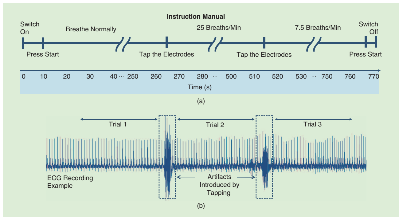
FIGURE 7. The recording instructions and an example of a recorded ECG. (a) The time sequence of the real-world ECG recordings. (b) Three trials at different breathing rates with transition periods in between. The unconstrained breathing (Trial 1, left) shows no obvious effects of the modulation of the ECG by respiration, while the ECG recorded while breathing at fixed rates (Trials 2 and 3, middle and right) shows clear effects of the RSA, a sinusoidal modulation of the ECG envelope by respiration.
