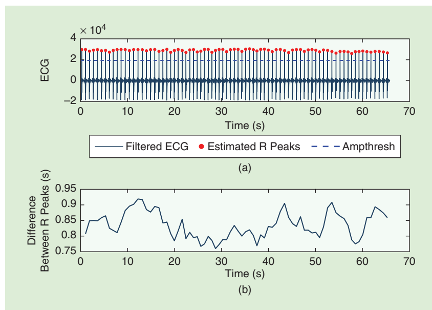
FIGURE 9. The detection of R-peaks in the ECG and the generation of HRV. (a) The band-passed filtered ECG and the suggested amplitude threshold (broken blue line). (b) The RRI obtained from the R-peak detection algorithm.
