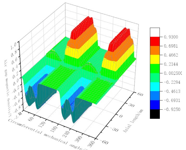
(a) Air gap magnetic density cloud map when there is no electric excitation.
