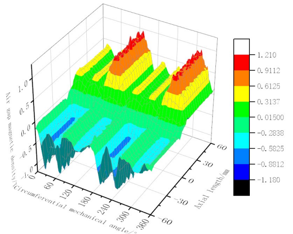
(c) Air gap magnetic density cloud map in flux weakened statement.
