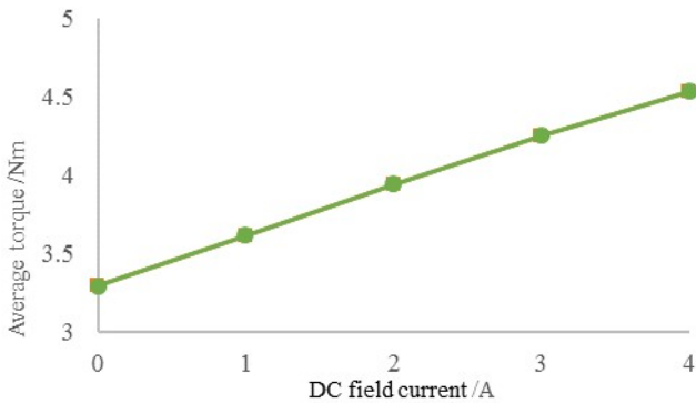
Fig. 11. Torque lifting capacity at low speed.
