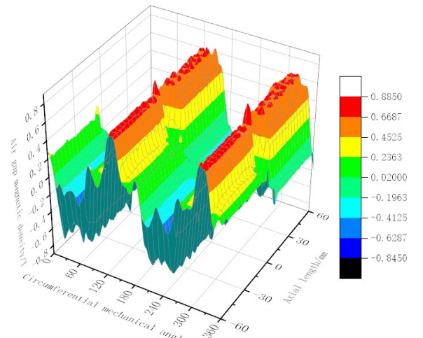
(b) Cloud map of air gap magnetic density in magnet enhancement statement.
