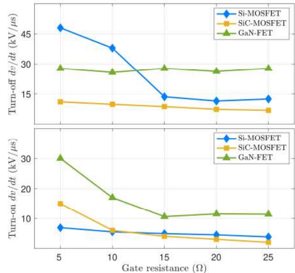
Fig. 18. Turn-off and turn-on dv/dt of Si-MOSFET, SiC-MOSFET, and cascode GaN-FET as the gate resistance is increased from 5 to 25 \Omega .
