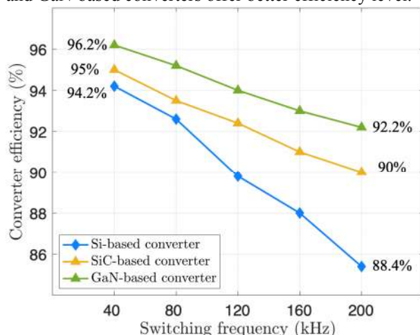
Fig. 28. Converter efficiency with different semiconductor device technologies as a function of increasing switching frequency from 40 to 200 kHz at an input voltage of 96 V.
