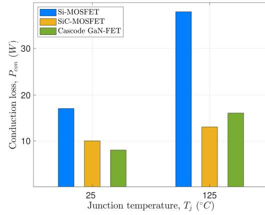
Fig. 9. Conduction loss of different devices at two junction temperatures.
