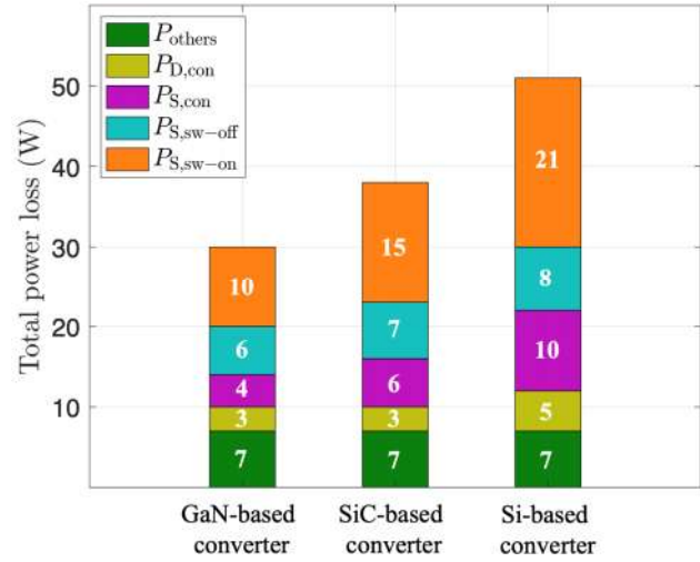
Fig. 26. Total power loss of each bidirectional converter.
