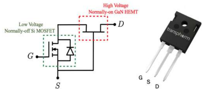
Fig. 5. A high voltage normally-on GaN HEMT with a low voltage normally-off Si MOSFET in a cascode configuration [54].
