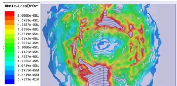
Fig.1. Eddy current loss of IPT system in marine environment (simulated by Ansys Maxwell with 5 A current, 60 mm distance, 100 mm diameter of coil, and the temperature 25°C).
