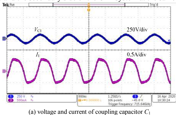
(a) voltage and current of coupling capacitor C_1
