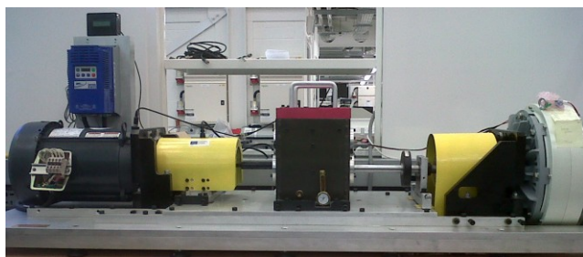
Fig. 6. Spectra Rig layout
