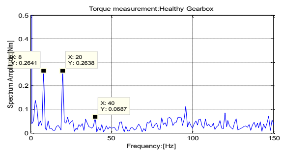
Fig 8.c) Load torque spectrum with healthy gearbox
