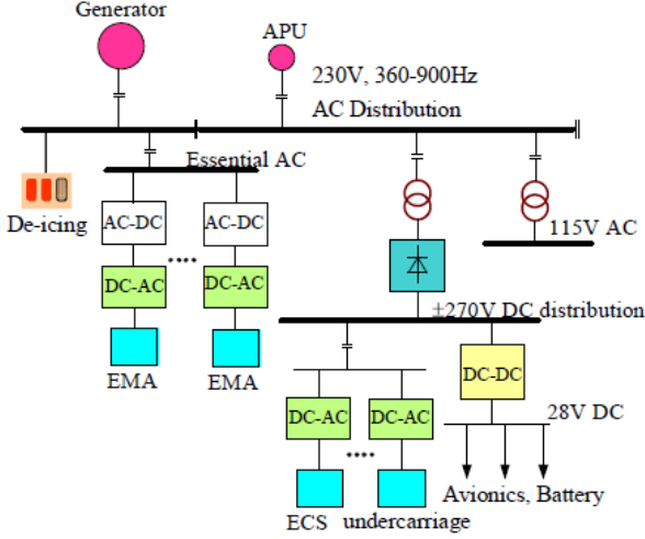
Fig. 1. The future power electrical systems for MEA
