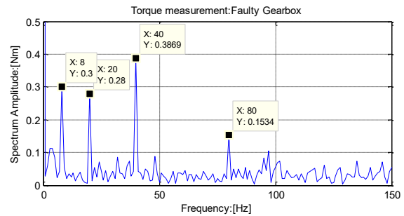
Fig. 8. a) Load torque spectrum with faulty gearbox
