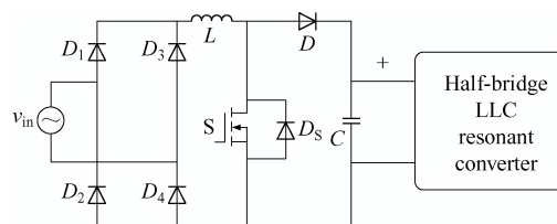
Fig. 11 LCD TV power supply of Boost PFC + half-bridge LLC resonant converter
