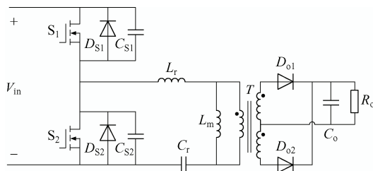
Fig. 6 The half-bridge LLC resonant converter topology
