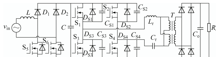
Fig. 14 OBC of bridgeless Boost PFC + full-bridge LLC resonant converter with double transformers
