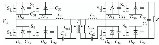
Fig. 16 OBC of Bi-LLC resonant converter
