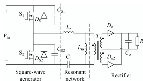
Fig. 1 The three parts of the LLC resonant converter
