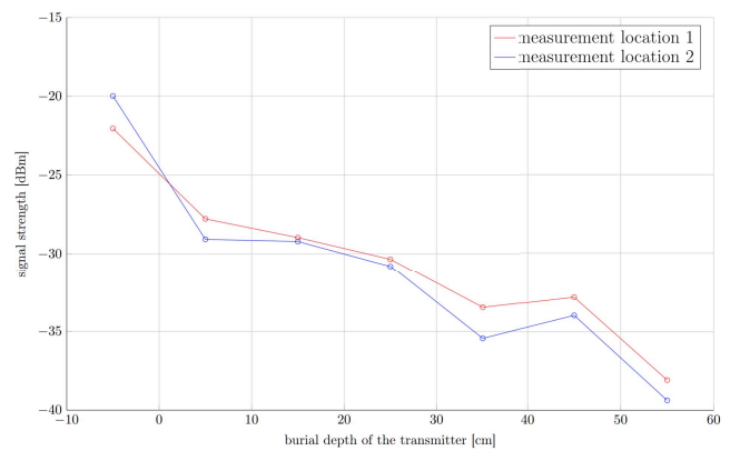
Fig. 4. Received signal strength for various depths
