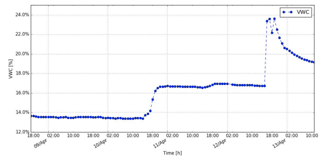
Fig. 5. Variation in volumetric water content (VWC) over five days
